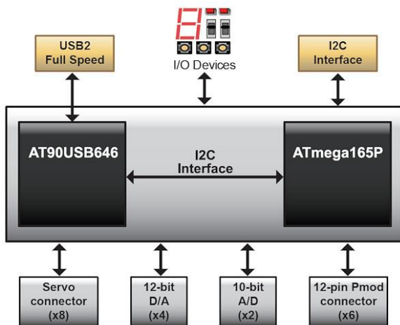
I/O Explorer USB block diagram.
