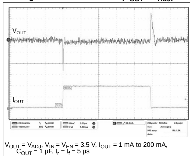
Figure 29. Load transient ( V_{OUT} = V_{ADJ} )
