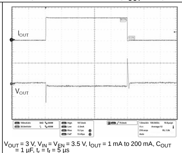
Figure 28. Load transient ( V_{OUT} = 3\text{ V} )
