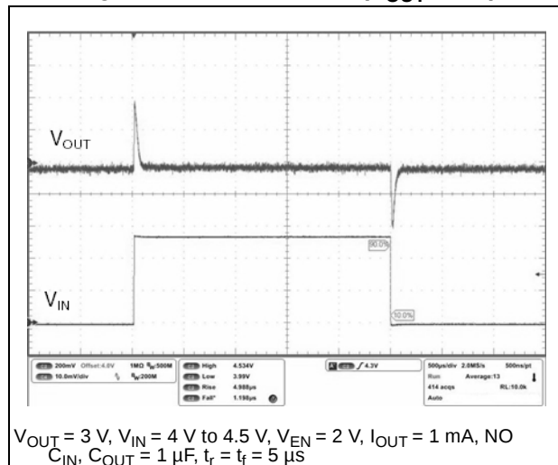
Figure 27. Line transient ( V_{OUT} = 3\text{ V} )
