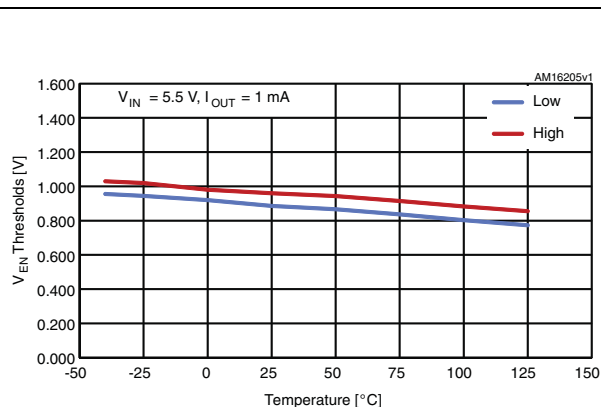
Figure 14. Enable pin thresholds vs. temp.
