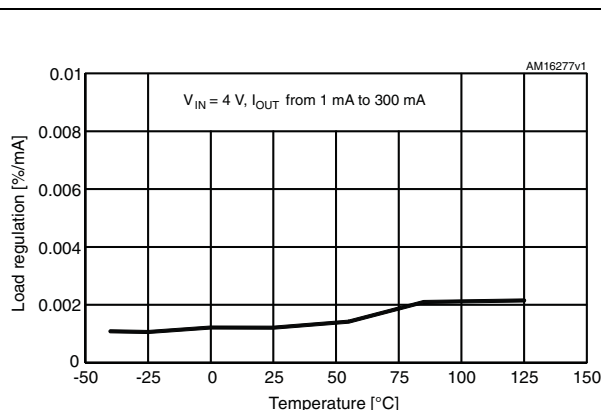
Figure 12. Load regulation vs. temp. for fixed version
