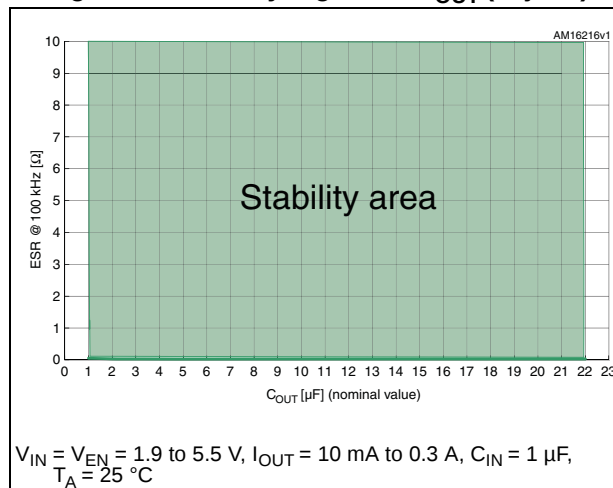
Figure 25. Stability region vs C_{OUT} (adjust.)
