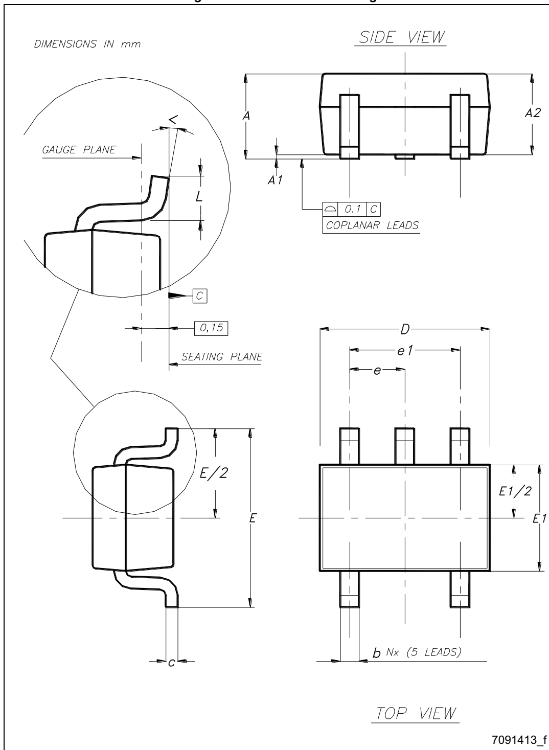
Figure 39. SOT323-5L drawing
