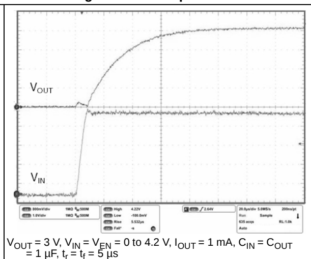
Figure 30. Startup transient
