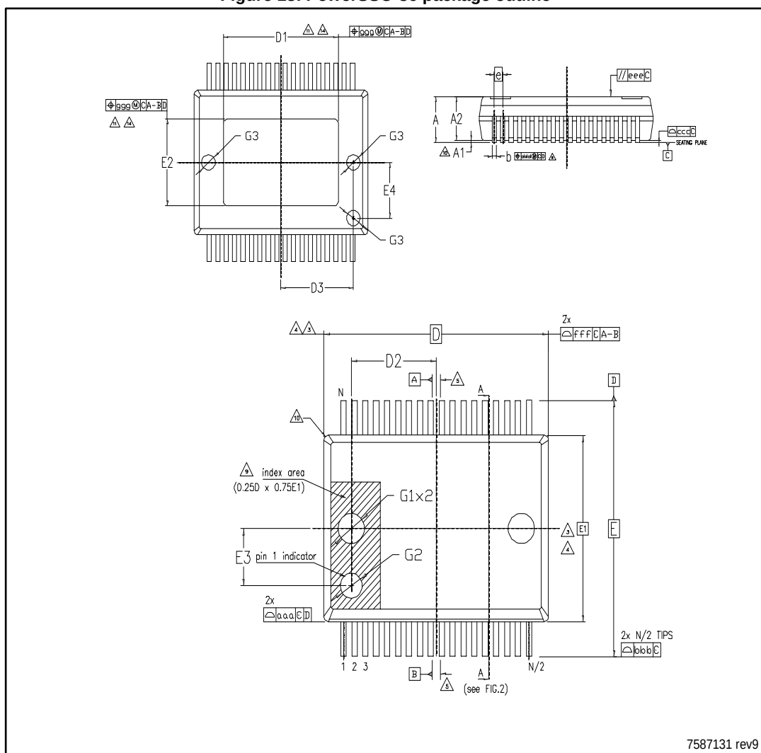
Figure 18: PowerSSO-36 package outline
