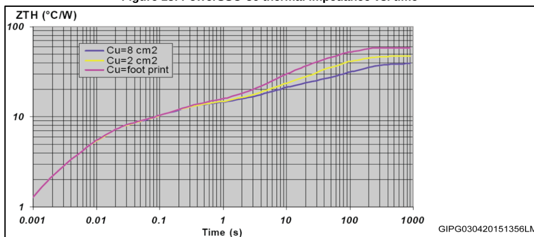
Figure 13: PowerSSO-36 thermal impedance vs. time
