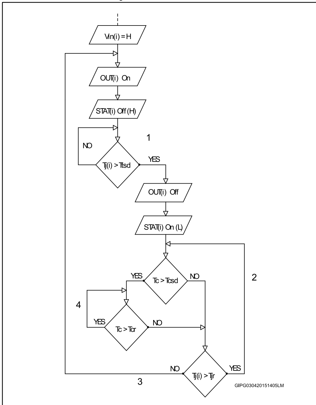
Figure 14: Thermal behavior
