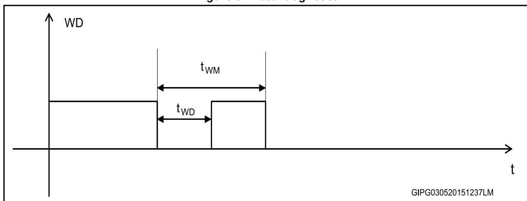
Figure 8: Watchdog reset
