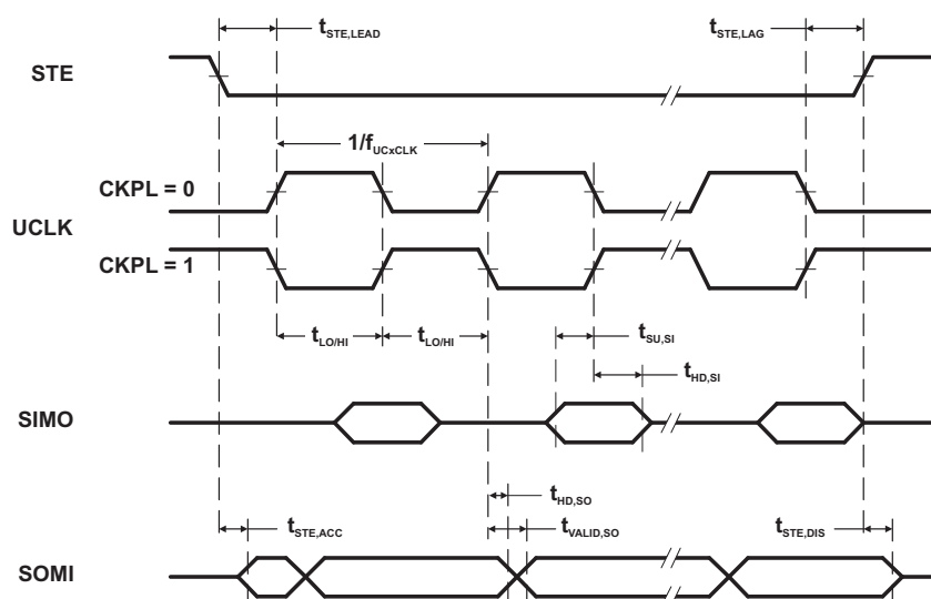
Figure 24. SPI Slave Mode, CKPH = 0
