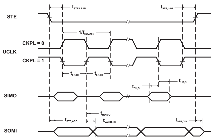
Figure 25. SPI Slave Mode, CKPH = 1
