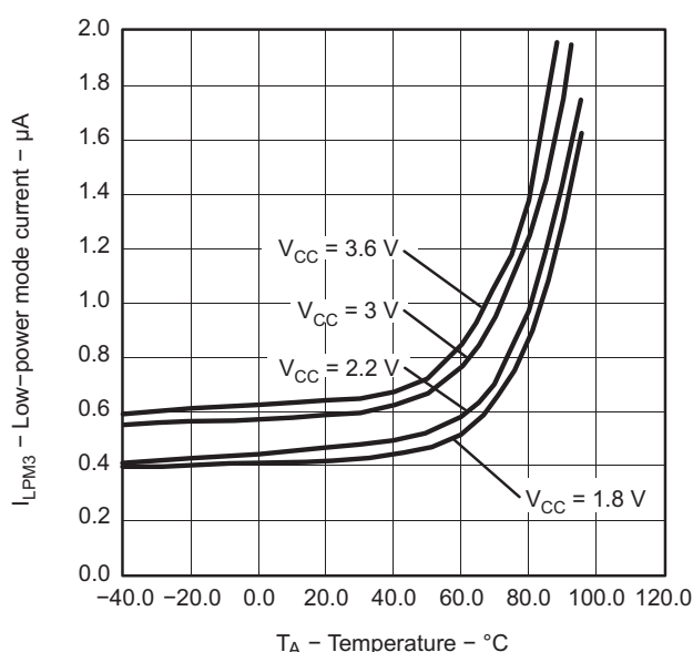
Figure 4. LPM3 Current vs Temperature
