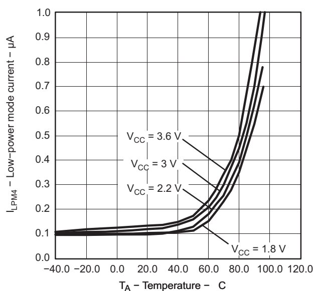
Figure 5. LPM4 Current vs Temperature
