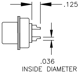
SIGNAL CONTACTS ACCEPTS UP TO 20 AWG WIRE
