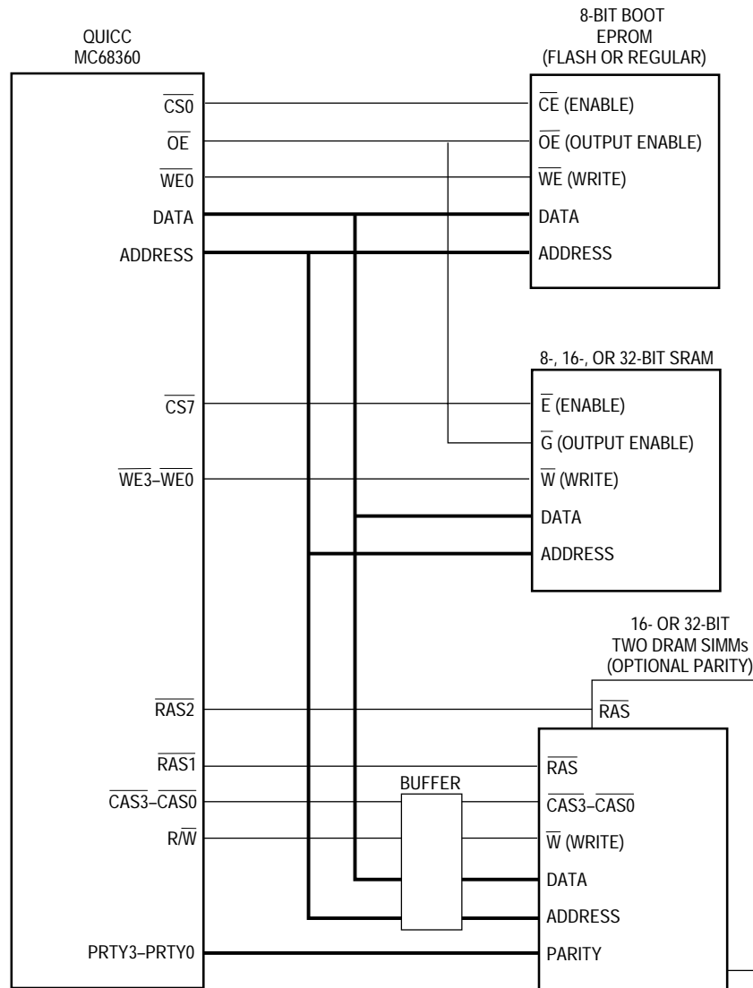
Figure 3. Larger QUICC System Configuration
