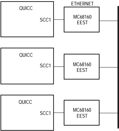
Figure 4. Ethernet LAN Capability
