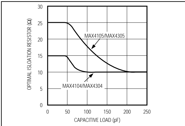
Figure 5. Optimal Isolation Resistor ( R_{ISO} ) vs. Capacitive Load
