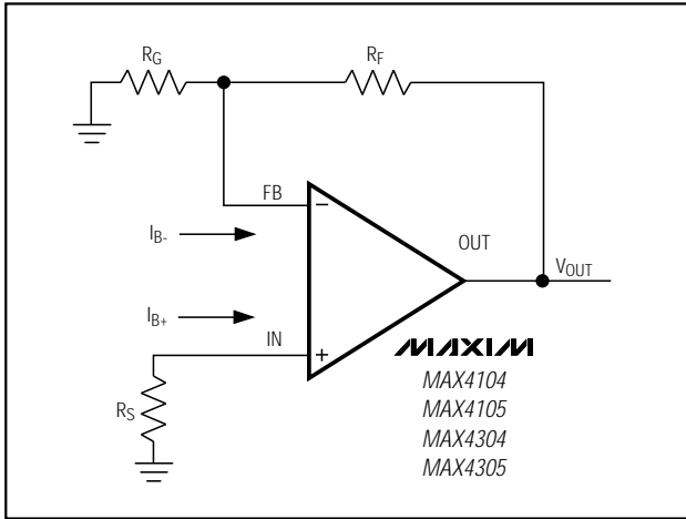
Figure 1. Output Offset Voltage
