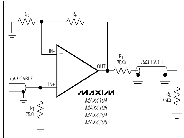
Figure 2. Video Line Driver
