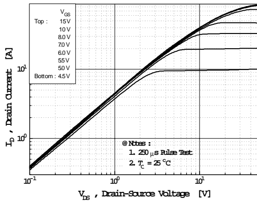
Fig 1. Output Characteristics
