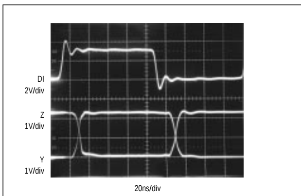
Figure 15. MAX3485E/MAX3490E/MAX3491E Driver Propagation Delay
