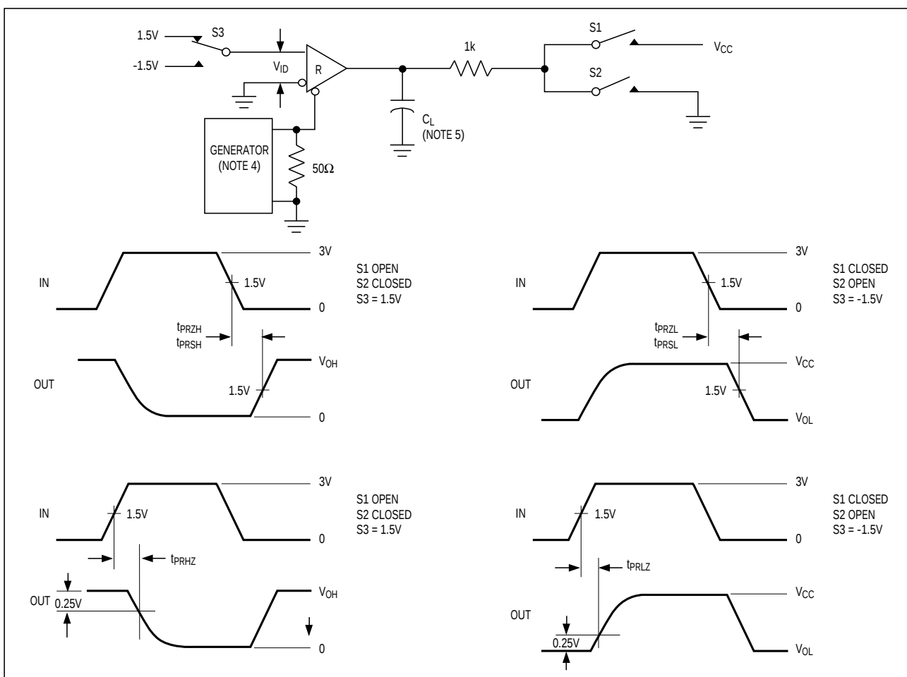
Figure 12. Receiver Enable and Disable Times
