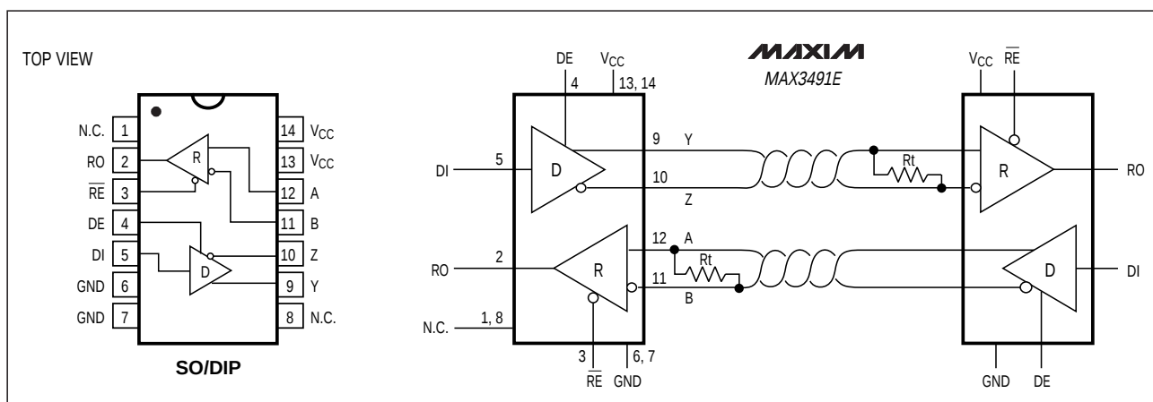
Figure 3. MAX3491E Pin Configuration and Typical Operating Circuit
