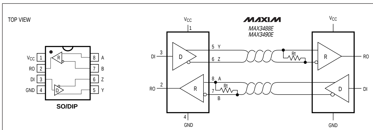
Figure 2. MAX3488E/MAX3490E Pin Configuration and Typical Operating Circuit
