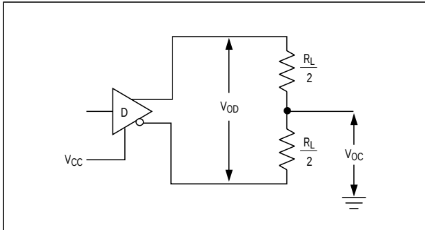
Figure 4. Driver V_{OD} and V_{OC}
