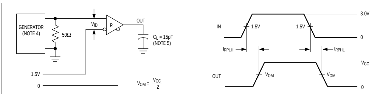
Figure 11. Receiver Propagation Delay
