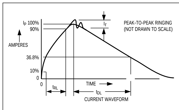
Figure 22b. Human Body Current Waveform
