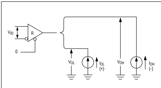
Figure 6. Receiver V_{OH} and V_{OL}
