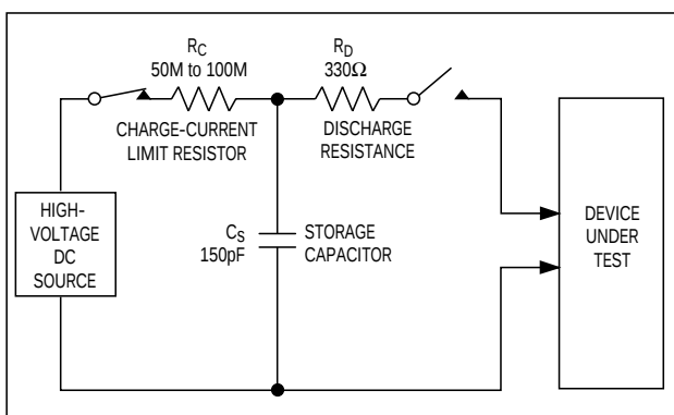
Figure 23a. IEC 1000-4-2 ESD Test Model
