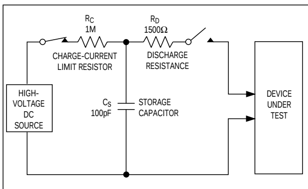
Figure 22a. Human Body ESD Test Model
