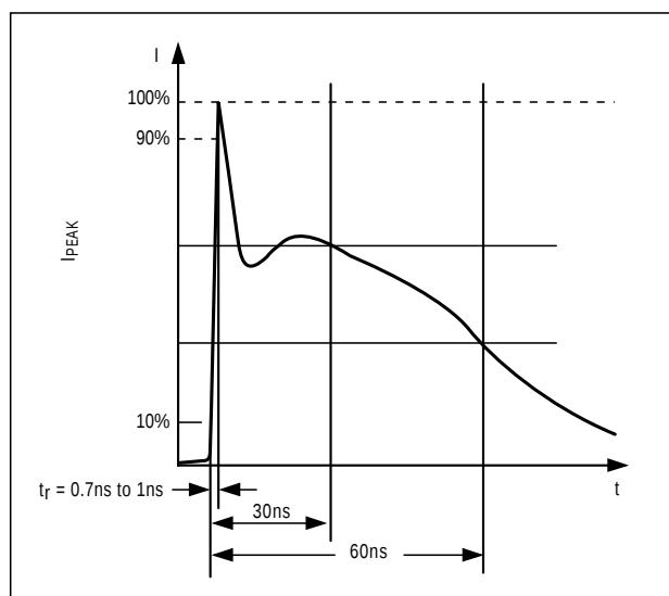
Figure 23b. IEC 1000-4-2 ESD Generator Current Waveform
