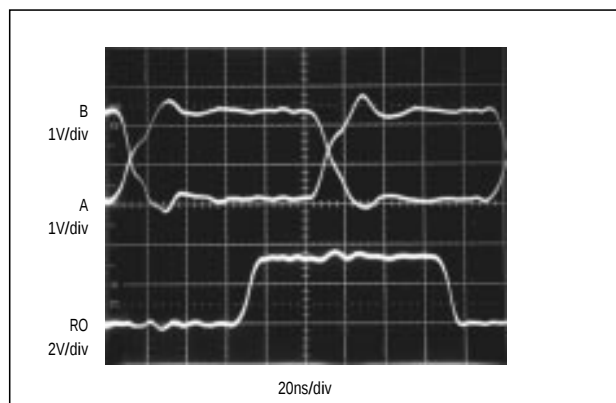
Figure 16. MAX3485E/MAX3490E/MAX3491E Receiver Propagation Delay Driven by External RS-485 Device
