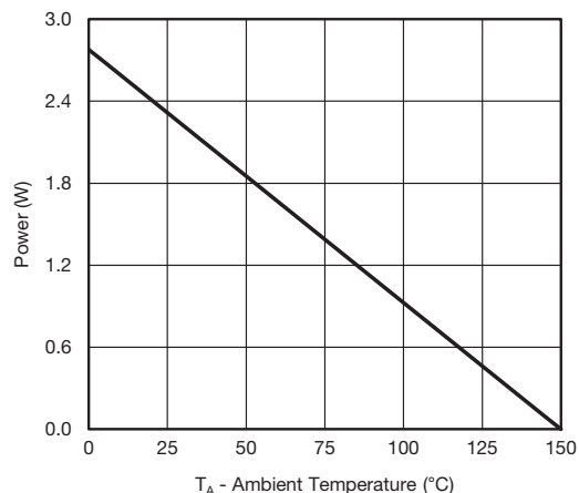
Power, Junction-to-Ambient
