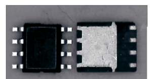
Standard SO-8 PowerPAK SO-8
