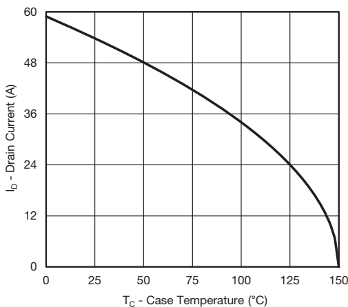
Current Derating*
