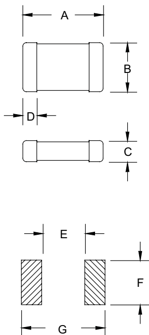
Pad Layout
