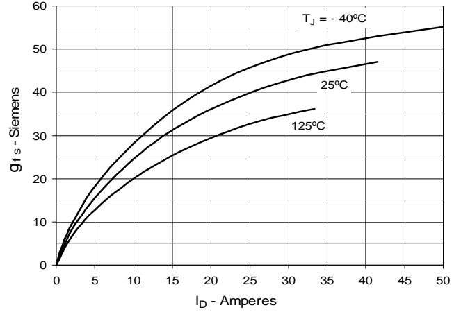
Fig. 8. Transconductance
