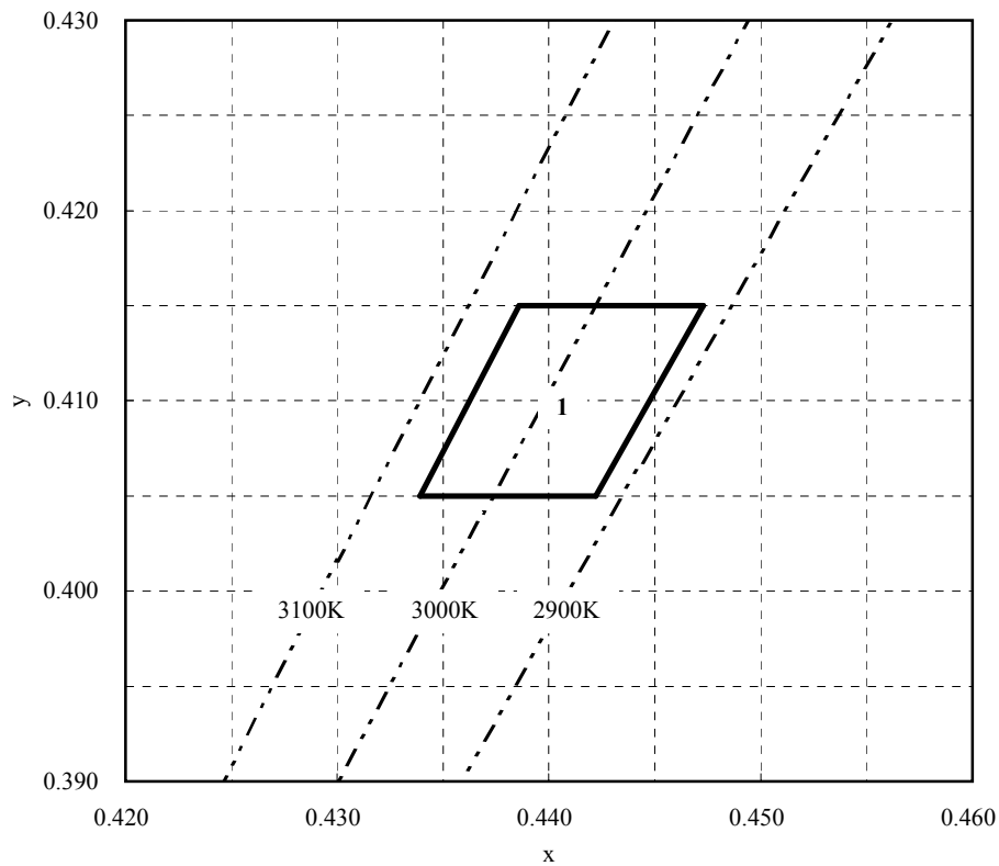
Chromaticity Diagram
