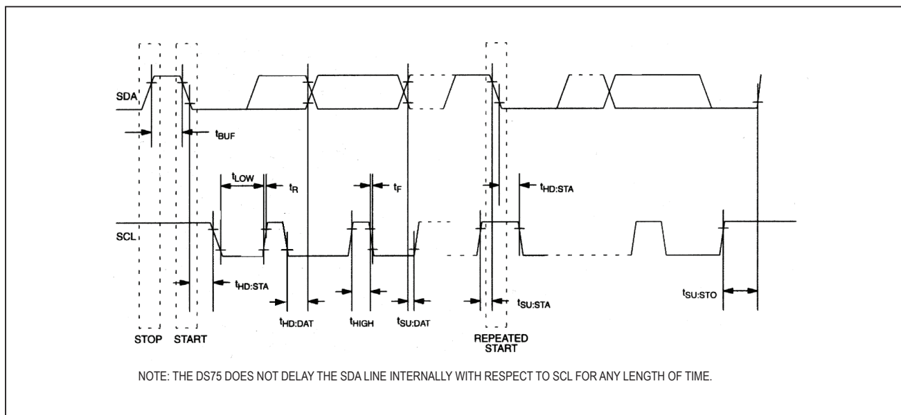
Figure 2. Timing Diagram
