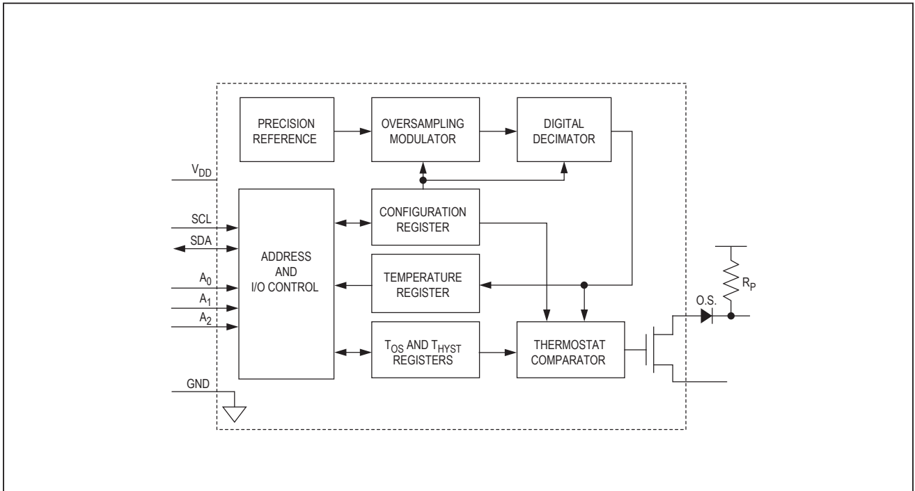
Figure 1. DS75S Functional Block Diagram
