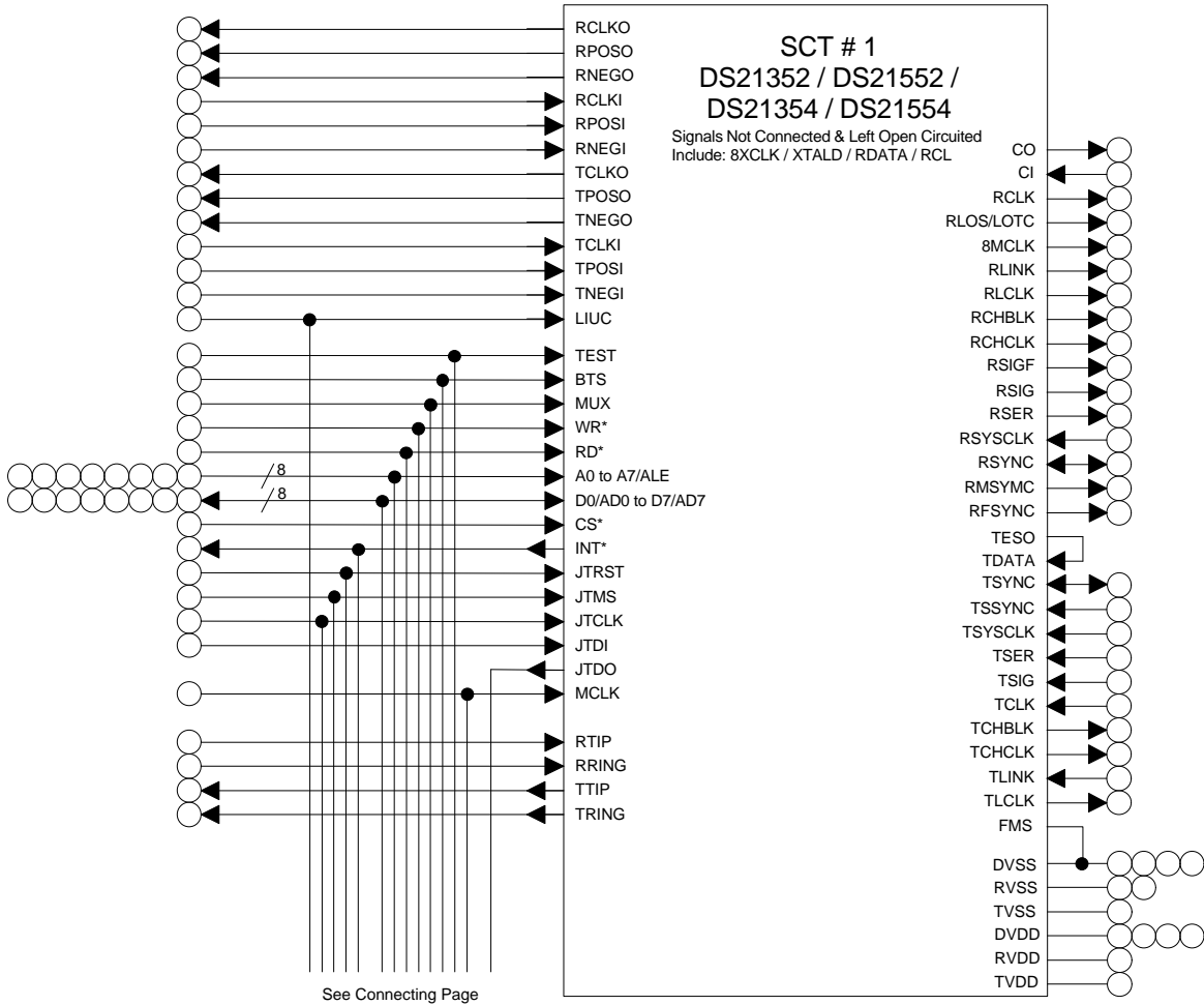
DS21Q352 / DS21Q552 / DS21Q354 / DS21Q554 Schematic Figure 1
