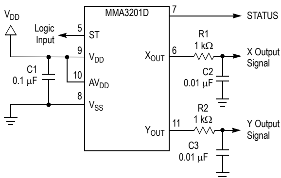
Figure 5. SOIC Accelerometer with Recommended Connection Diagram
