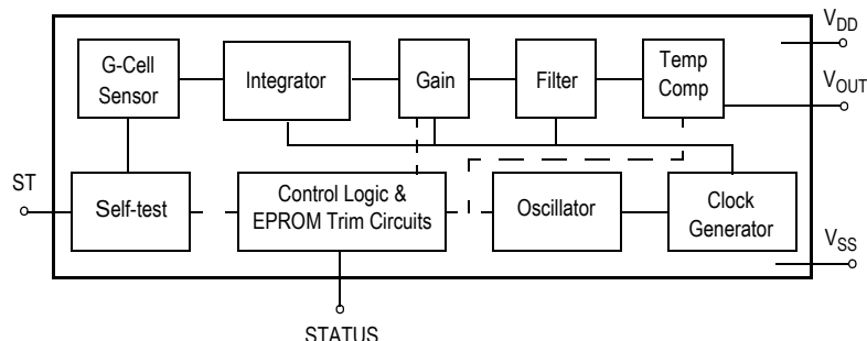
Figure 1. Simplified Accelerometer Functional Block Diagram
