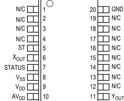
Figure 2. Pin Connections
