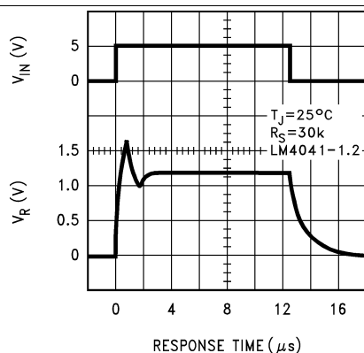
Figure 5. Start-Up Characteristics
