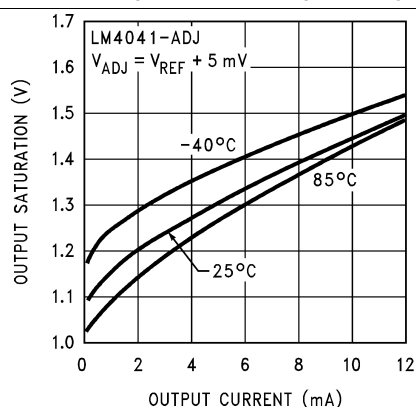
Figure 9. Output Saturation (SOT-23 Only)
