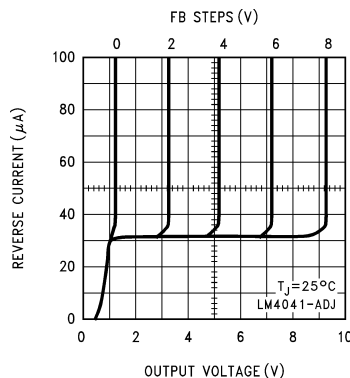
Figure 21. Reverse Characteristics
