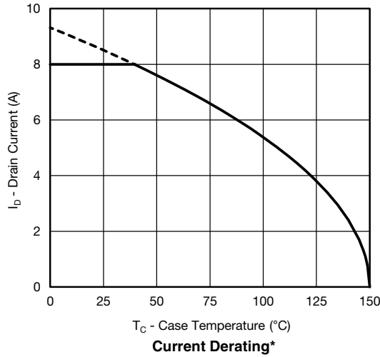
Current Derating*
