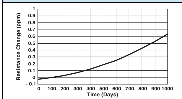
FIGURE 1 - SHELF LIFE - VHA518-11 12K9 VS. QHE
