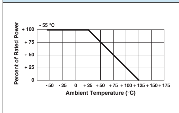
FIGURE 4 - POWER DERATING CURVE
