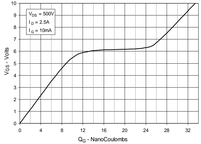
Fig. 10. Gate Charge
