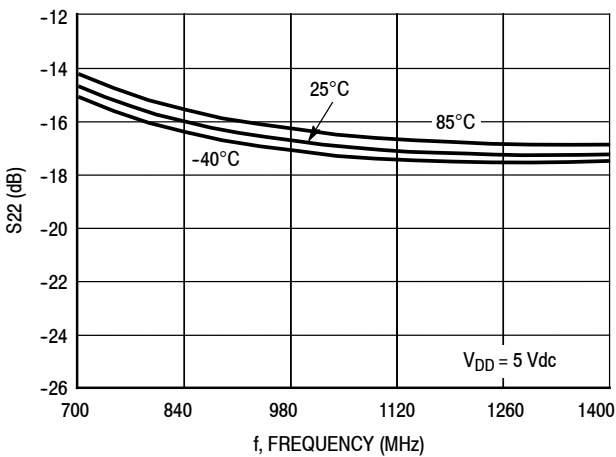
Figure 7. S22 versus Frequency versus Temperature
