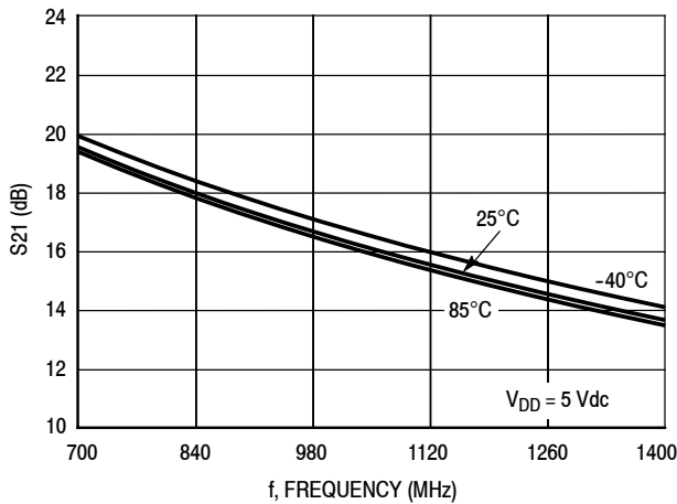
Figure 6. S21 versus Frequency versus Temperature
