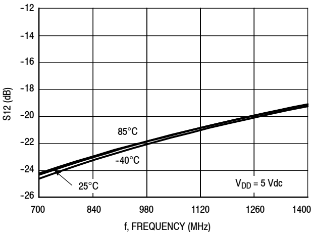
Figure 5. S12 versus Frequency versus Temperature
