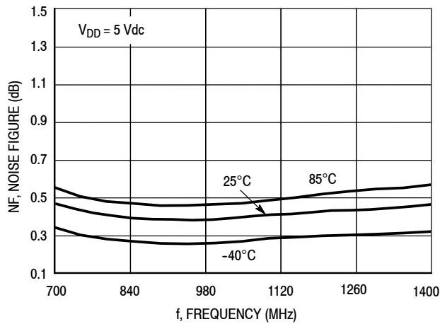
Figure 8. Noise Figure versus Frequency versus Temperature
