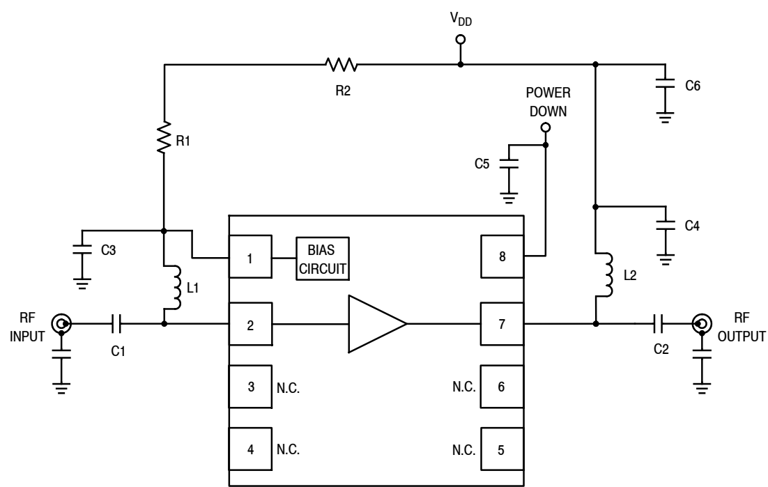
Figure 2. MML09231H Test Circuit Schematic
