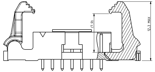
SECTION C - C EXAMPLE 10078993-G02-14YLF LOW PROFILE LATCH
