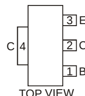
TOP VIEW Pin Out Configuration
