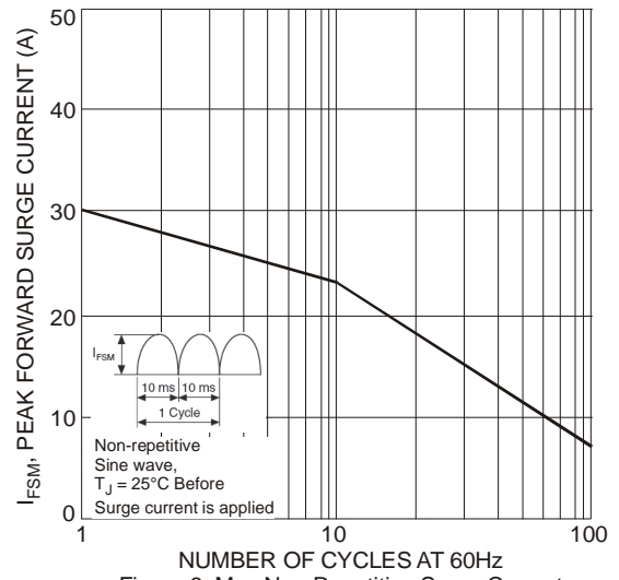
Figure 6 Max Non-Repetitive Surge Current
