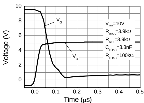
Switch-Off Speed
