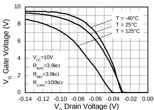
Transfer Characteristic
