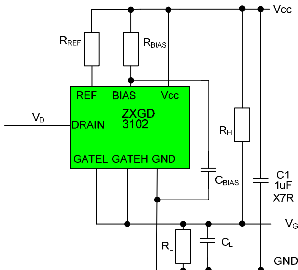
Figure 4: Test Circuit
