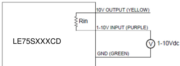
Dimming Configuration using External Voltage
