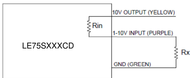
Dimming Configuration using External Resistance
