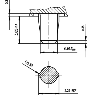
DETAIL OF CENTRAL PEG SCALE 8/1
