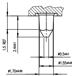
DETAIL OF LOCATING PEGS (2x) SCALE 8/1
