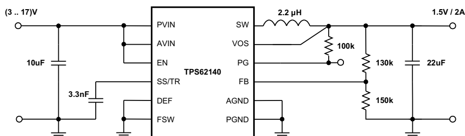
Figure 47. 1.5-V/2-A Power Supply
