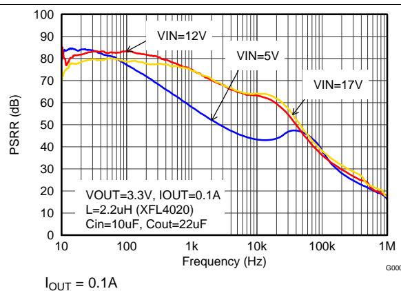
Figure 29. Power-Supply Rejection Ratio, f_{SW} = 2.5 MHz
