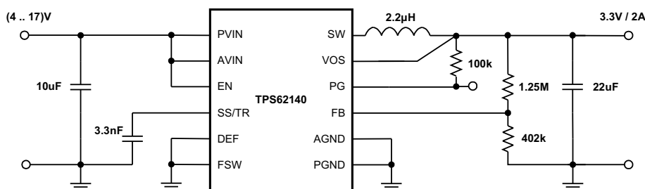
Figure 7. 3.3V/2A Step-Down Converter
