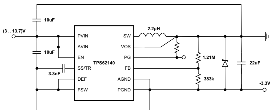
Figure 42. -3.3V Inverting Power Supply
