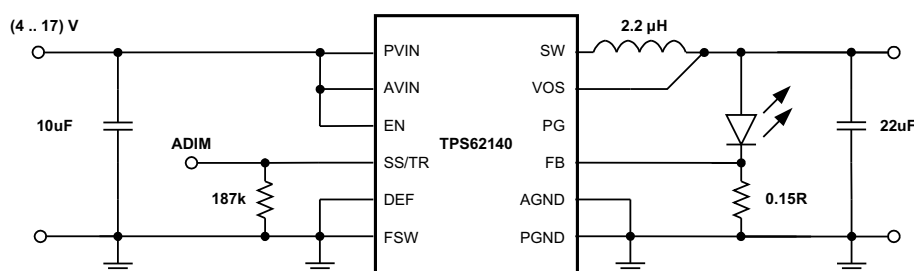
Figure 40. Single Power LED Supply
