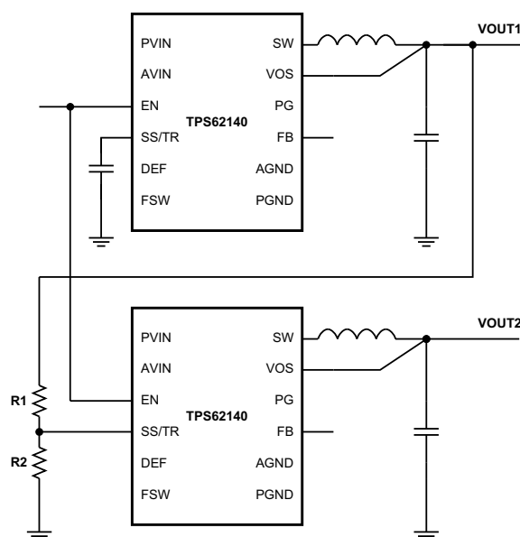
Figure 9. Sequence for Ratiometric and Simultaneous Startup
