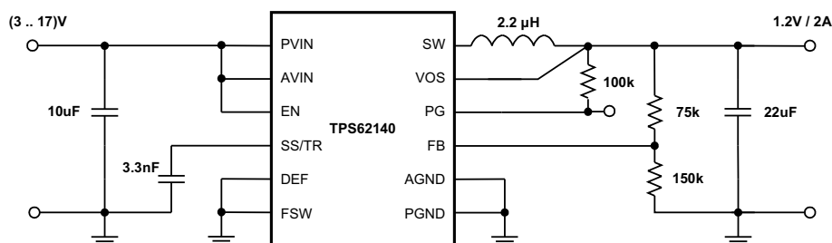
Figure 48. 1.2-V/2-A Power Supply
