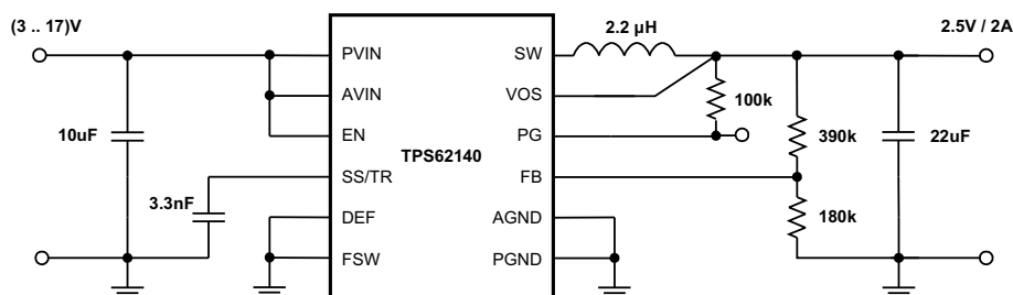
Figure 45. 2.5-V/2-A Power Supply
