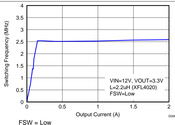
Figure 25. Switching Frequency
