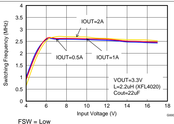
Figure 24. Switching Frequency
