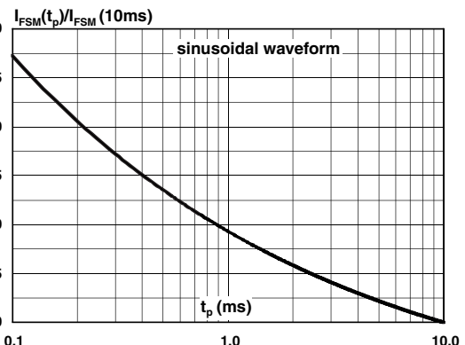
Figure 10. Relative variation of non-repetitive peak surge forward current versus pulse duration
