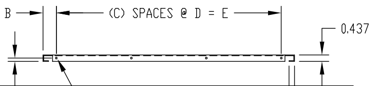
VENTILATED TOP OR BOTTOM COVER TBC-14262 & TBC-14263
