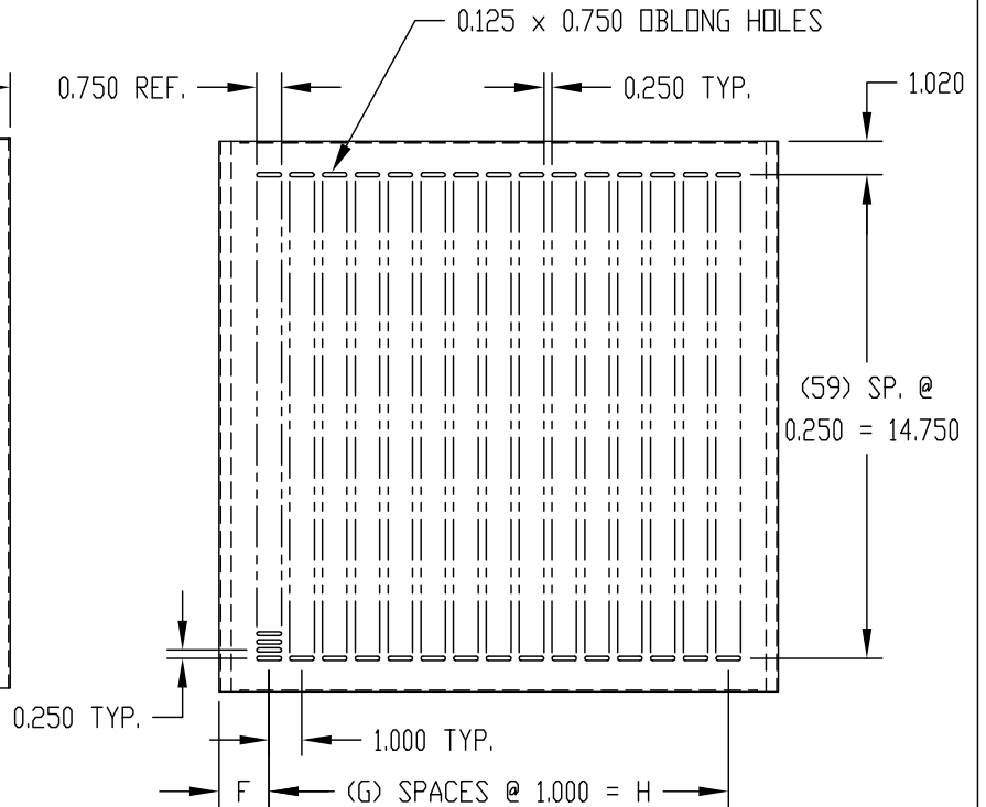
VENTILATED TOP OR BOTTOM COVER TBC-14262 & TBC-14263
