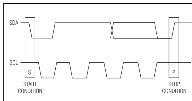
Figure 3. START and STOP Conditions
