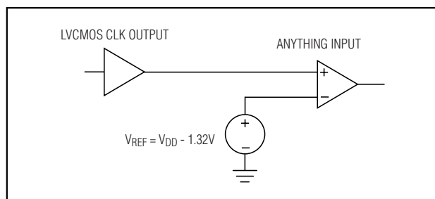
Figure 2. Connecting LVCMOS Output to LVPECL Input
