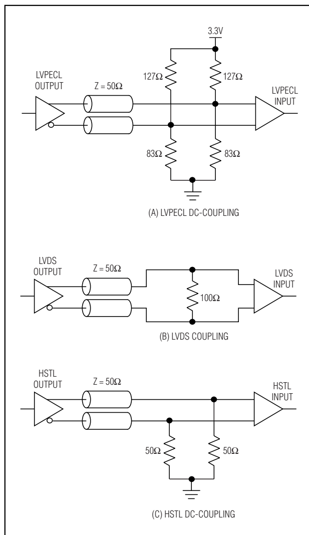
Figure 1. DC LVPECL, LVDS, and HSTL Termination
