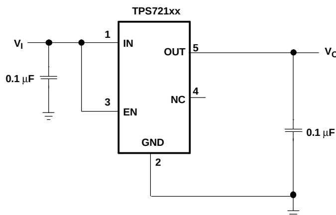
Figure 18. Typical Application Circuit
