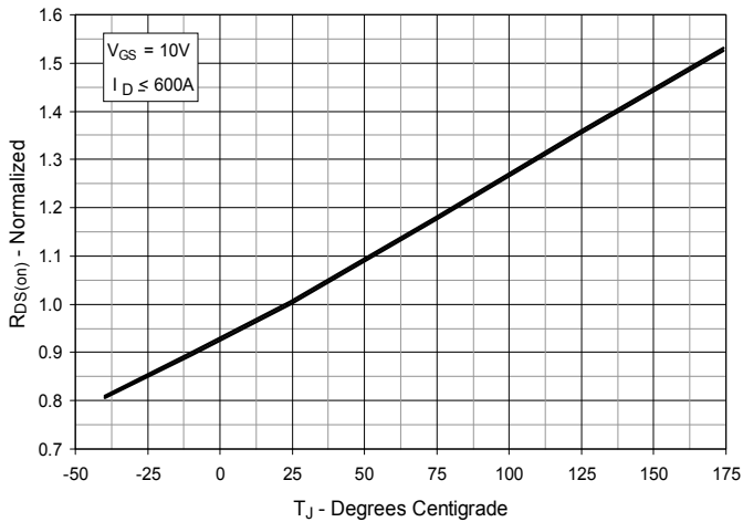
Fig. 3. Normalized R_{DS(on)} vs. Junction Temperature
