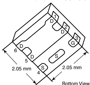
PowerPAK SC-70-6L-Single
