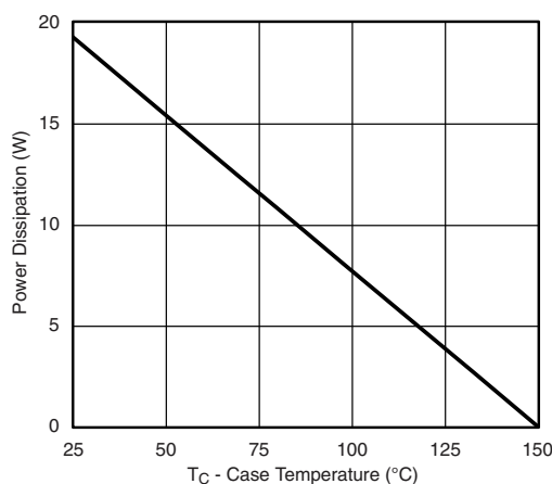
Power, Junction-to-Case
