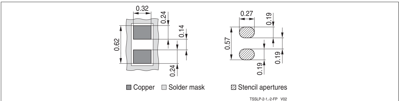
Figure 10 TSSLP-2-4 Footprint
