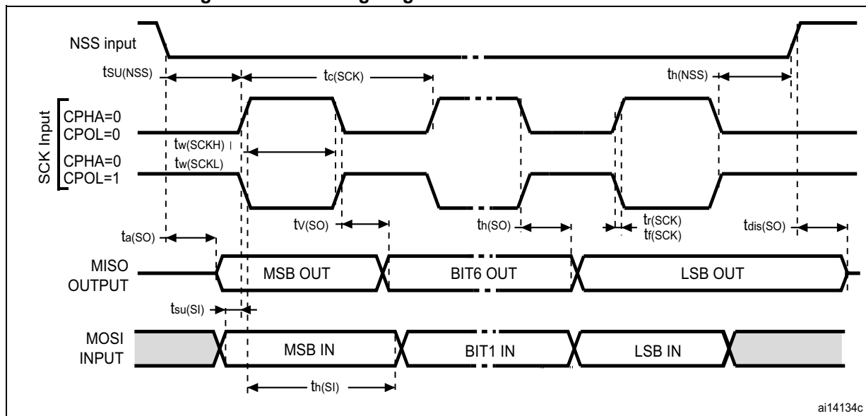
Figure 19. SPI timing diagram - slave mode and CPHA = 0
