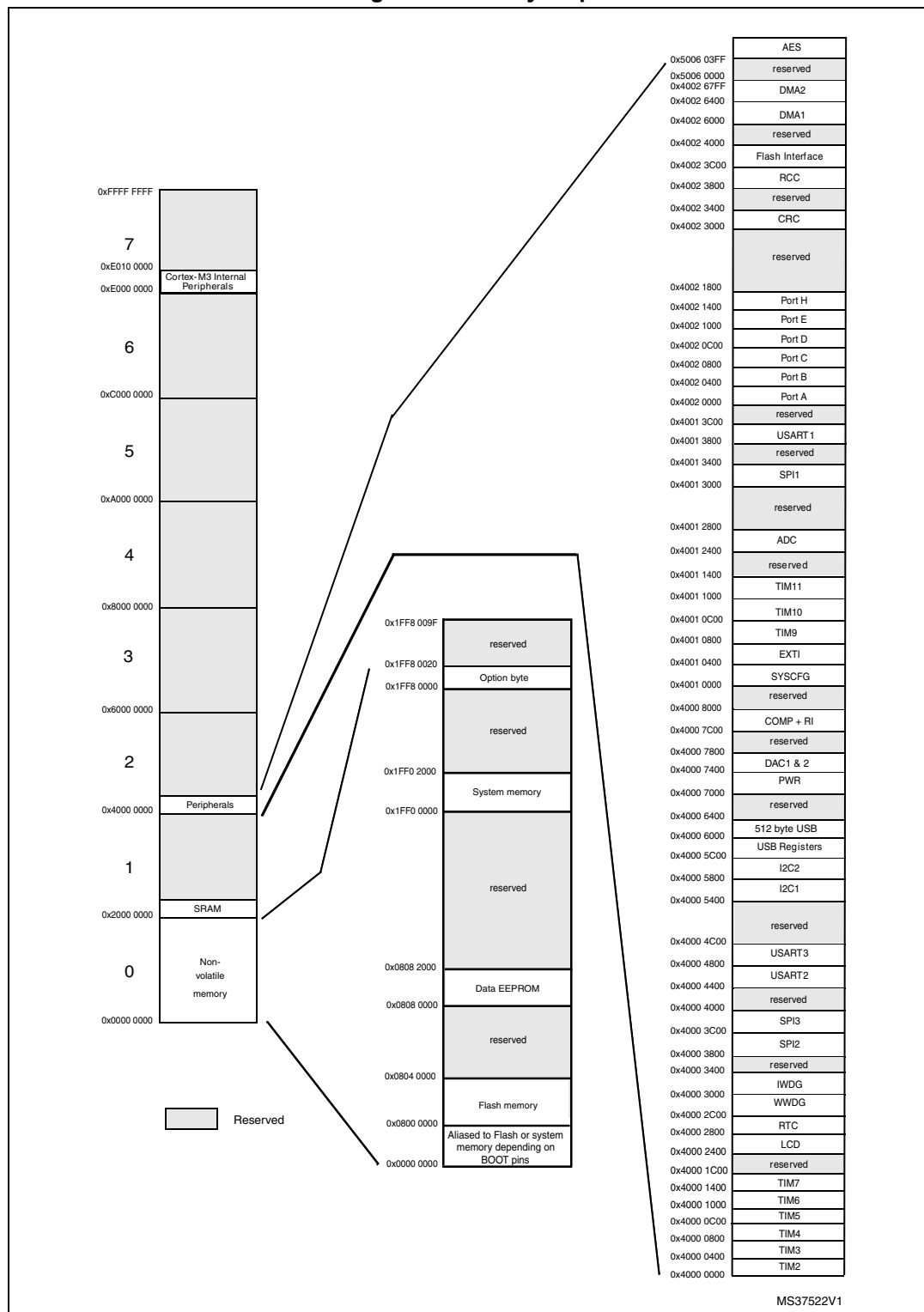
Figure 6. Memory map
