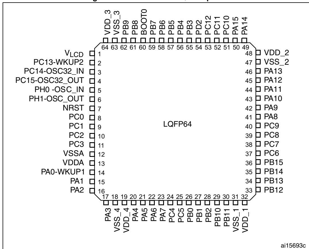
Figure 5. STM32L162RC LQFP64 pinout
