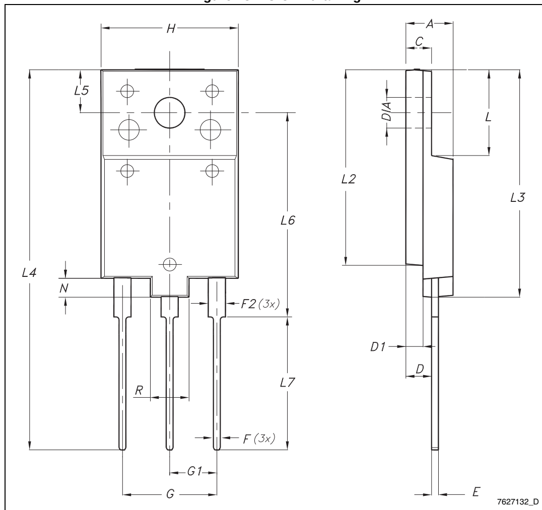
Figure 28. TO-3PF drawing
