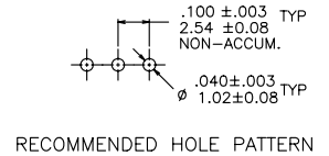
RECOMMENDED HOLE PATTERN
