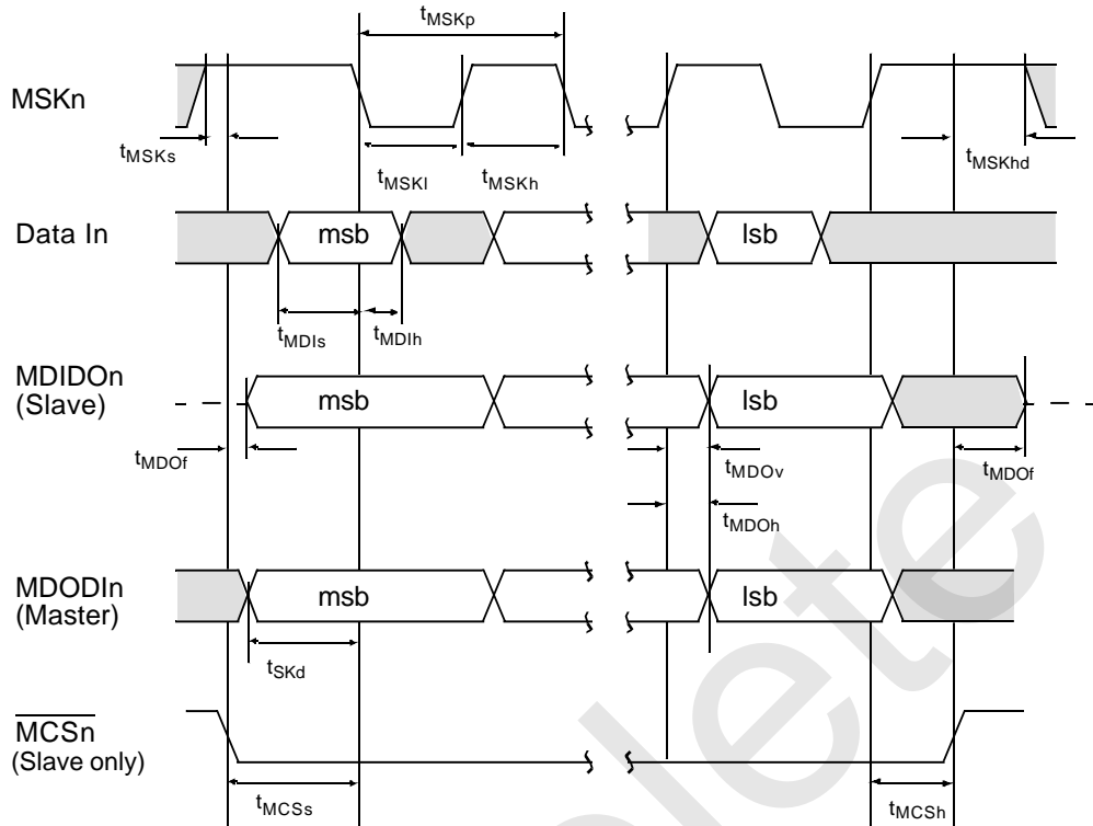
Figure 86. MICROWIRE Transaction Timing, Alternate Mode, MIDL bit = 1
