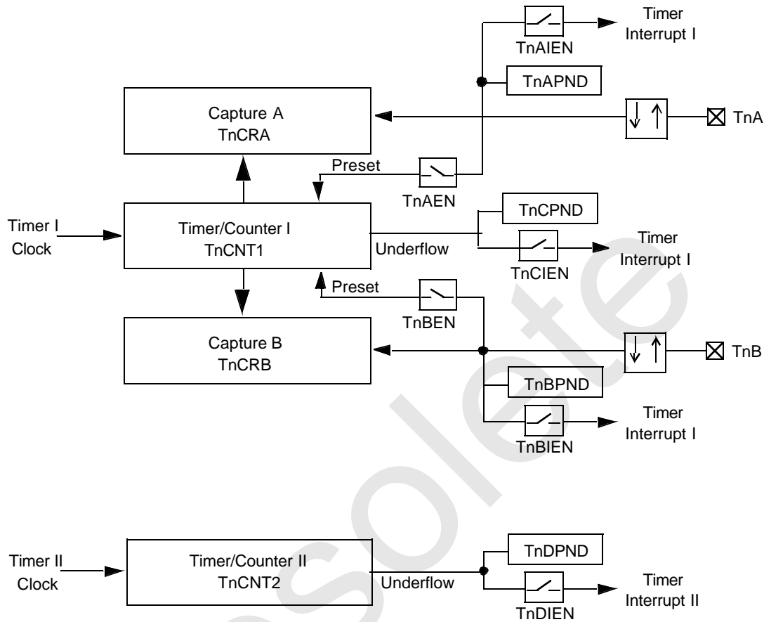
Figure 15. Mode 2: Dual Input Capture Block Diagram
