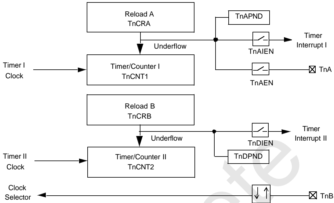
Figure 16. Mode 3: Dual Independent Timer/Counter Block Diagram
