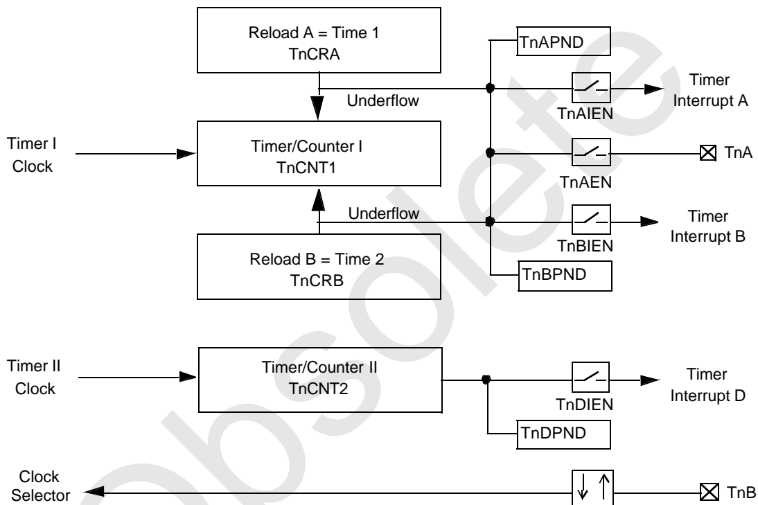
Figure 14. Mode 1: Processor-Independent PWM Block Diagram
