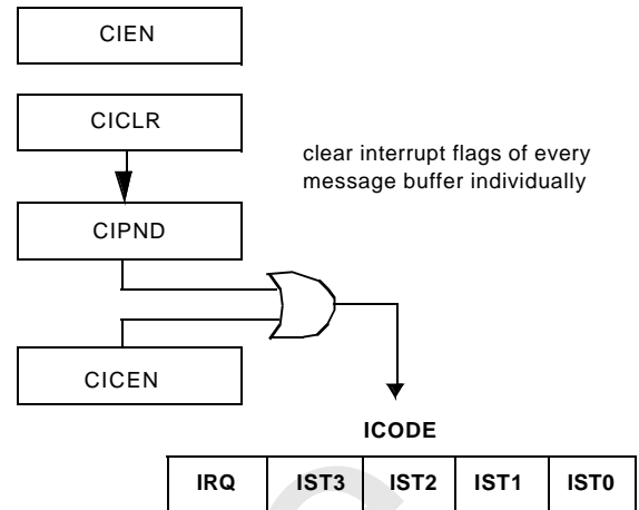
Figure 67. CR16CAN Interrupt Management
