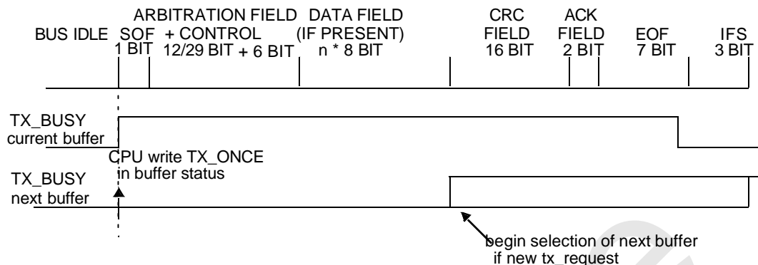
Figure 64. Data Transmission
