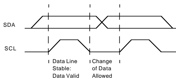
Figure 39. Bit Transfer
