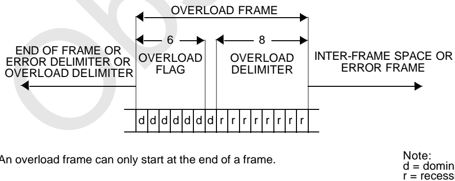
Figure 49. CAN Overload Frame
