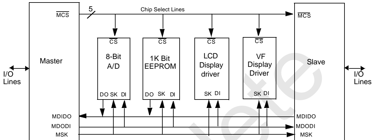
Figure 24. MICROWIRE Interface
