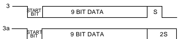
Figure 37. Nine Data Bit Frame Options
