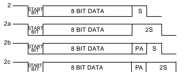
Figure 36. Eight Data Bit Frame Options
