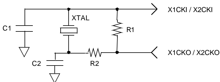
Figure 8. External Crystal Network
