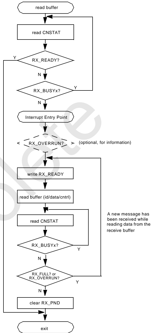
Figure 62. Buffer Read Routine (BUFFLOCK Disabled)
