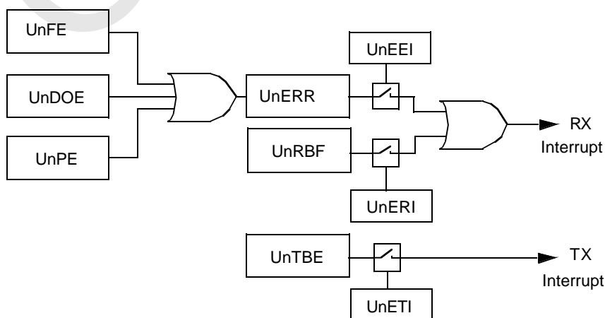
Figure 38. USART Interrupts
