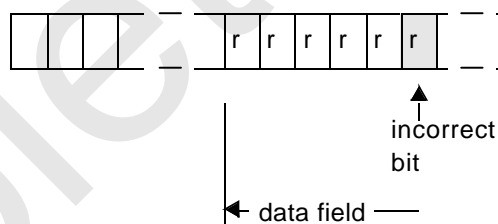
Figure 71. EBID Example
