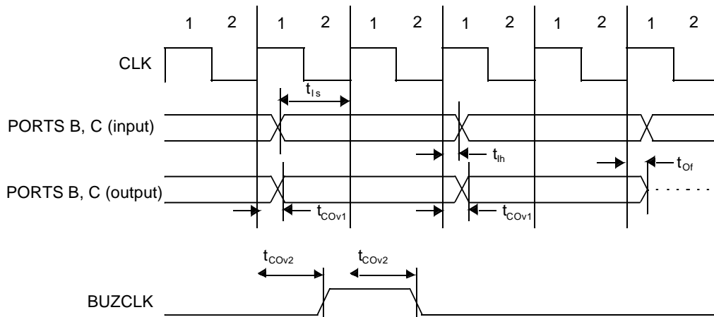
Figure 82. Port Signals Timing
