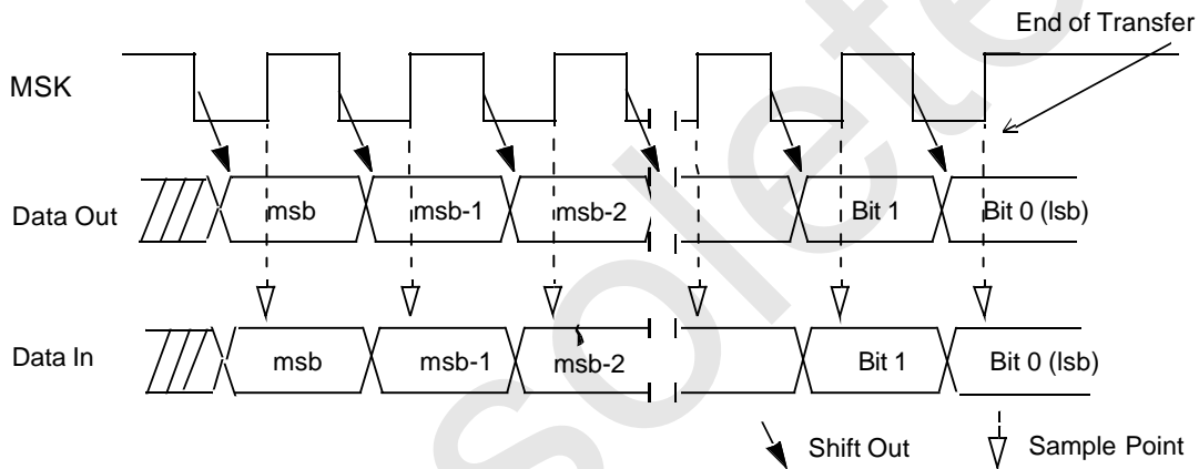
Figure 27. Normal Mode, MIDL Bit = 1
