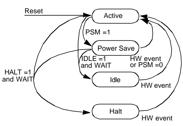
Figure 6. Power Modes and Transitions
