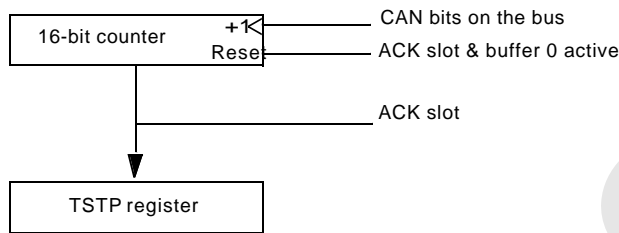
Figure 68. Time Stamp Counter
