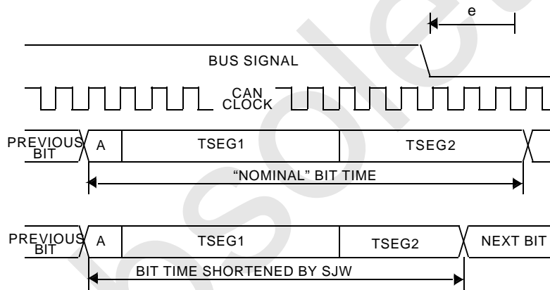
Figure 54. Re-synchronization (e < -SJW)
