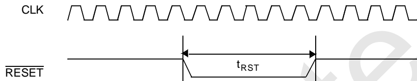
Figure 79. Non-Power-On Reset
