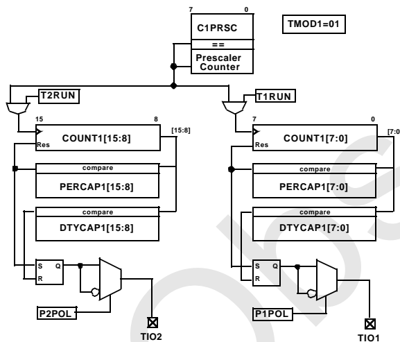
Figure 20. VTU Dual 8-bit PWM Mode
