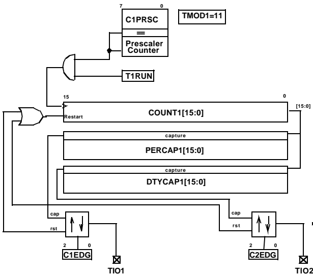
Figure 22. VTU Dual 16-bit Capture Mode
