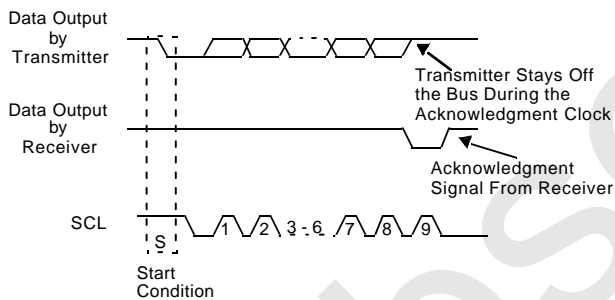
Figure 42. ACCESS.bus Acknowledge Cycle
