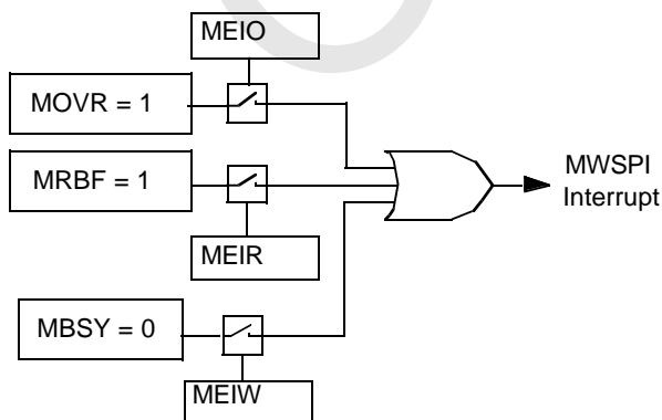
Figure 30. MWSPI Interrupts
