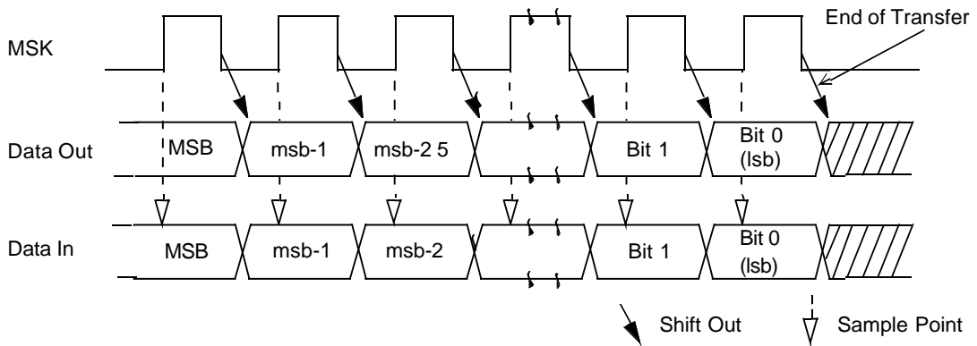
Figure 26. Normal Mode, MIDL Bit = 0
