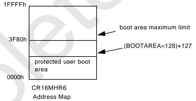
Figure 4. Memory Protection through BOOTAREA
