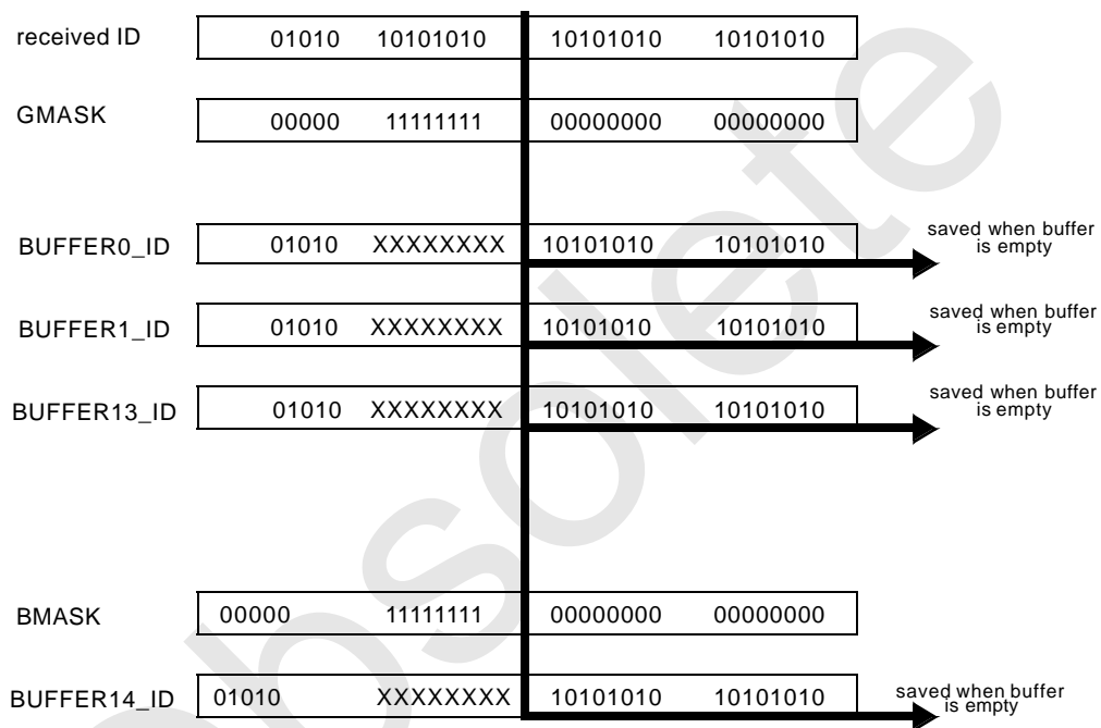
Figure 59. Message Storage with BUFFLOCK Enabled
