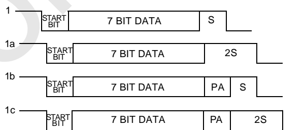
Figure 35. Seven Data Bit Frame Options
