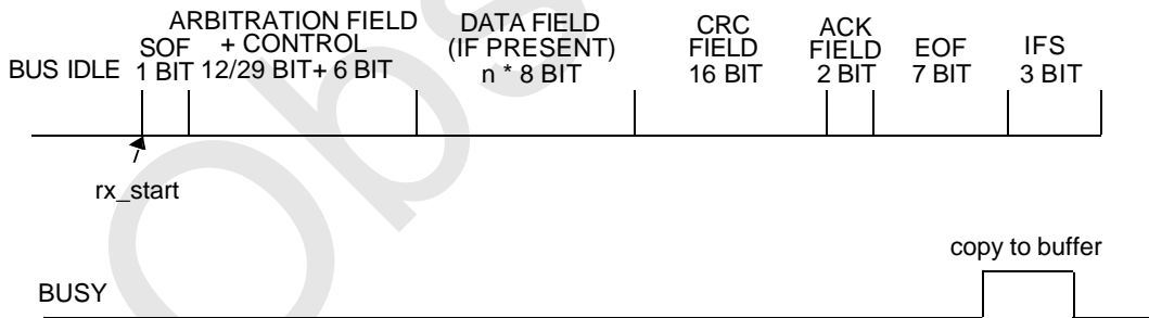
Figure 61. Receive Timing
