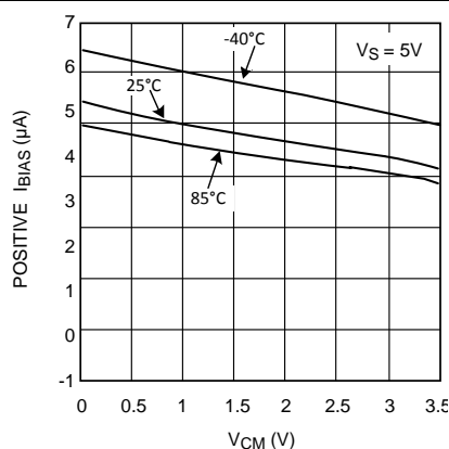
Figure 12. Bias Current vs. Common Mode Voltage
