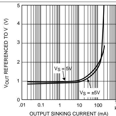
Figure 35. Output Sinking Current
