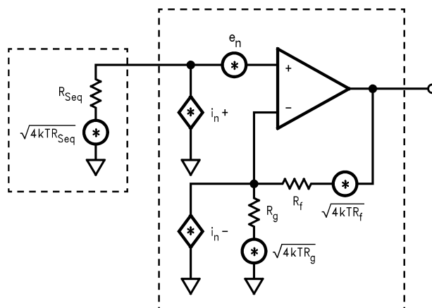
Figure 44. Non-Inverting Amplifier Noise Model
