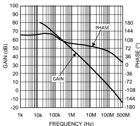
Figure 40. Open Loop Gain and Phase vs. Frequency
