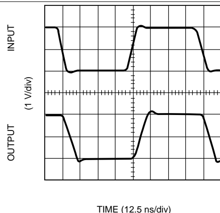
Figure 18. Non-Inverting Large Signal Pulse Response ( V_S = \pm 5\text{ V} )
