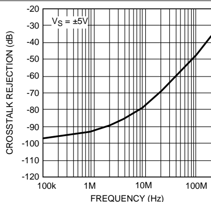
Figure 38. CrossTalk vs. Frequency (LMH6655 only)
