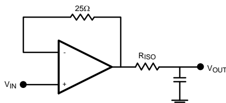
Figure 41. Isolation Resistor Placement
