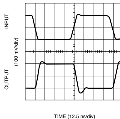
Figure 21. Inverting Small Signal Pulse Response ( V_S = 5\text{ V} )
