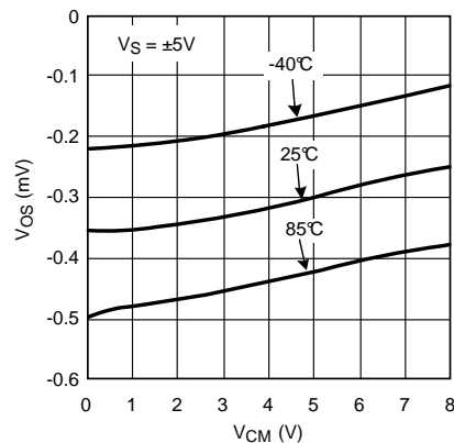
Figure 9. Offset Voltage vs. Common Mode
