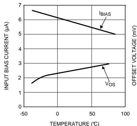
Figure 11. Bias Current and Offset Voltage vs. Temperature
