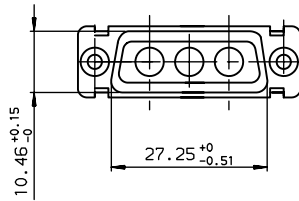
LAYOUT DIMENSIONS (after plating) CONNECTOR SIDE VIEW
