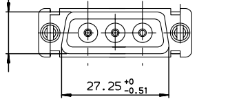
LAYOUT DIMENSIONS (after plating) CONNECTOR SIDE VIEW
