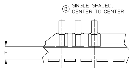
TAPE MOUNTING DETAIL
