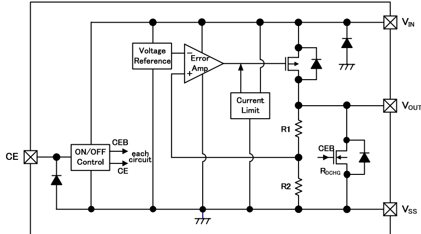
XC6504 Series, Type A
