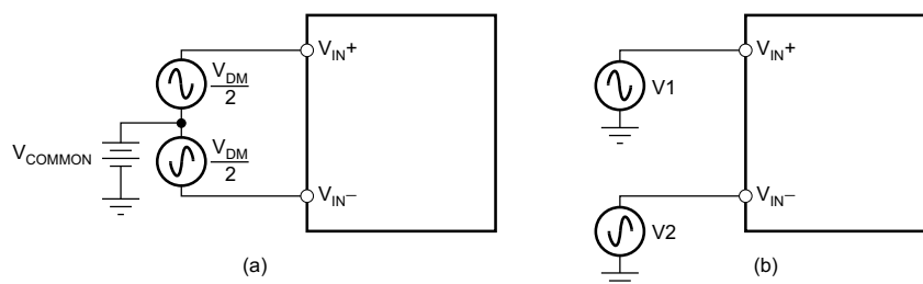
Figure 81. Fully-Differential Analog Input
