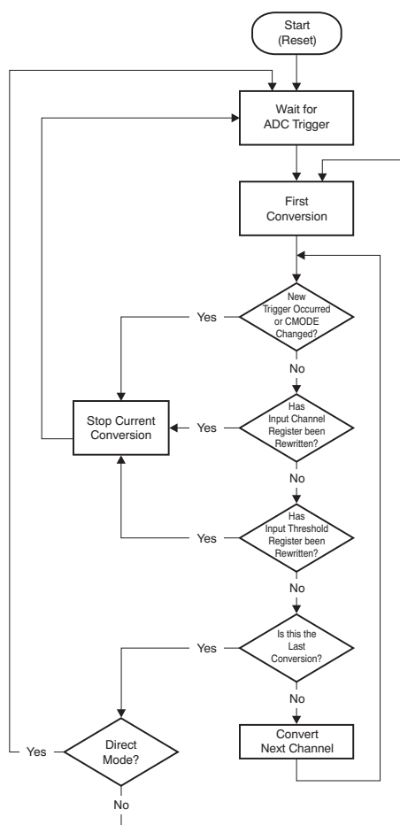
Figure 82. ADC Conversion Sequence
