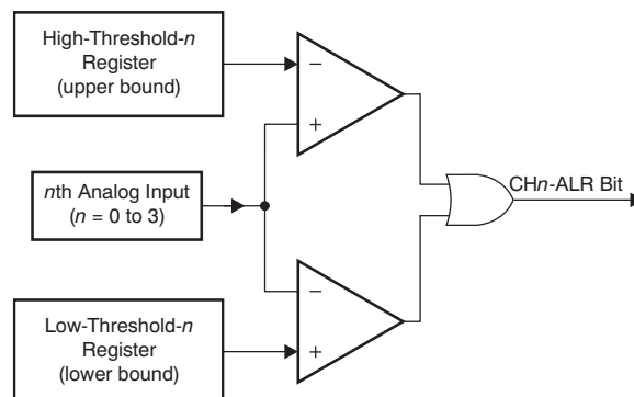
Figure 95. CH n Out-of-Range Alarm
