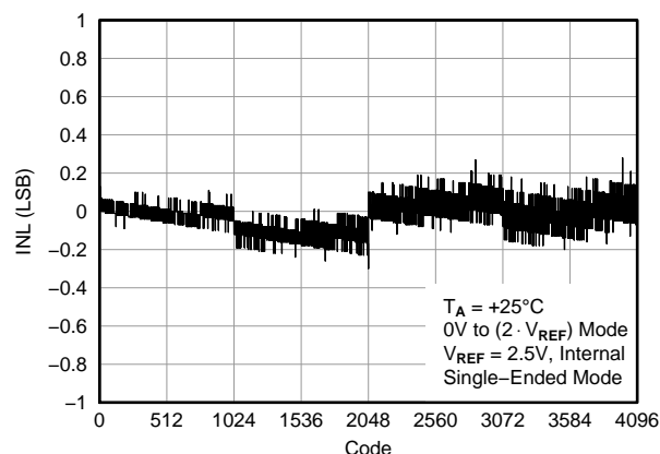
Figure 46. LINEARITY ERROR vs CODE
