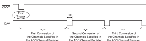
Figure 85. ADC External Trigger
