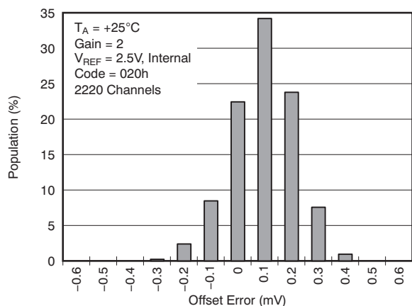
Figure 26. OFFSET VOLTAGE
