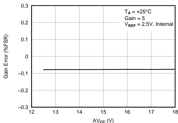
Figure 25. GAIN ERROR vs SUPPLY
