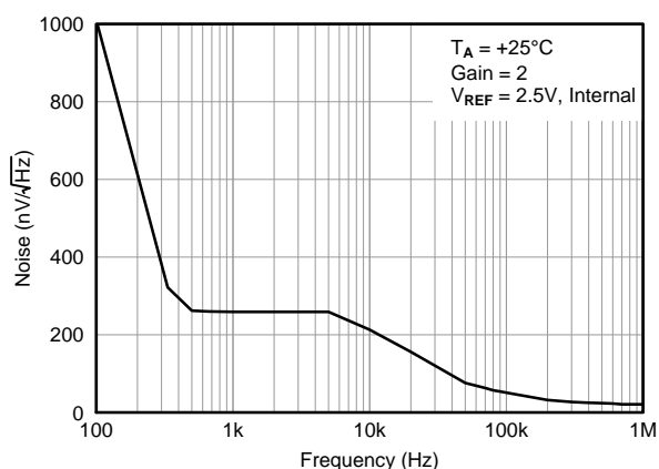
Figure 73. INTERNAL REFERENCE NOISE vs FREQUENCY
