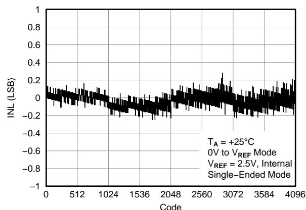
Figure 44. LINEARITY ERROR vs CODE
