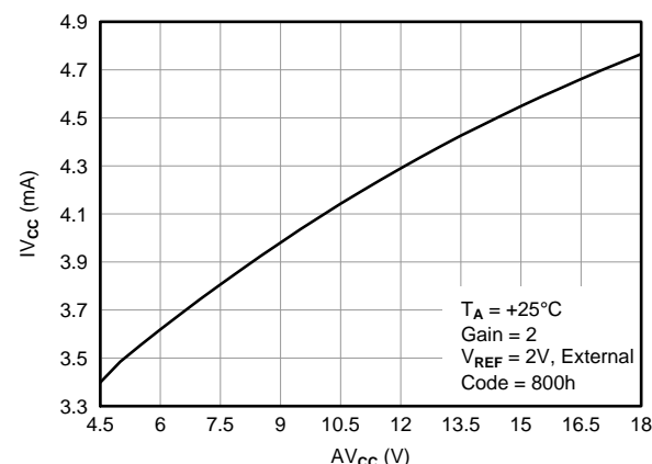
Figure 35. DAC SUPPLY CURRENT vs DAC SUPPLY VOLTAGE
