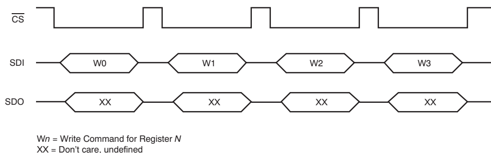
Figure 106. Write Operation in Standalone Mode
