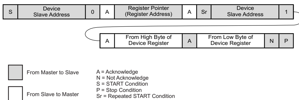
Figure 102. Read a Single Word
