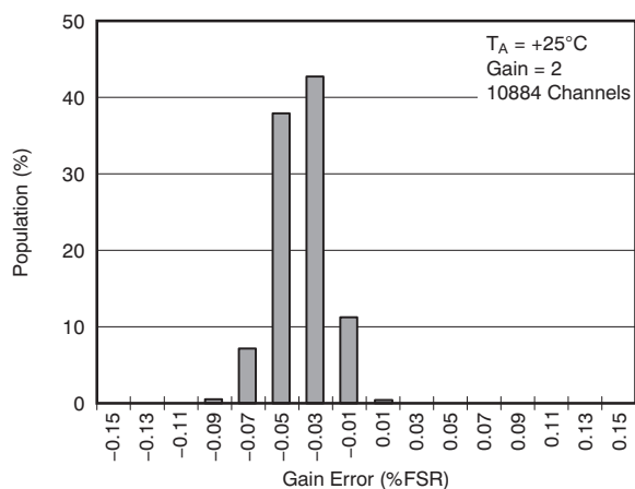
Figure 20. GAIN ERROR
