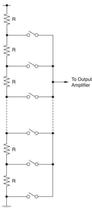
Figure 92. Resistor String
