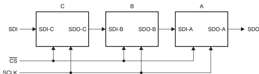
Figure 108. Three AMC7812Bs in a Daisy-Chain Configuration
