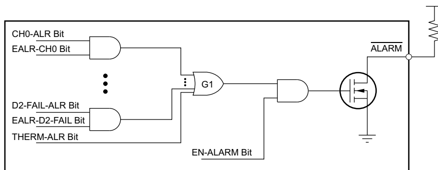
Figure 97. \overline{\text{ALARM}} Pin
