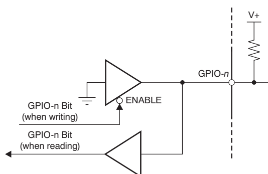
Figure 99. GPIO Pins
