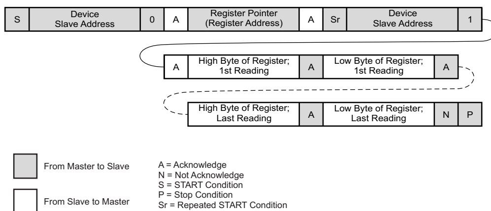
Figure 103. Read Multiple Words
