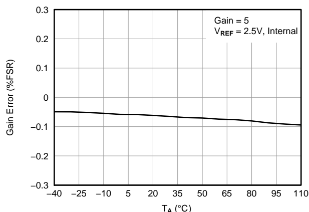
Figure 23. GAIN ERROR vs TEMPERATURE
