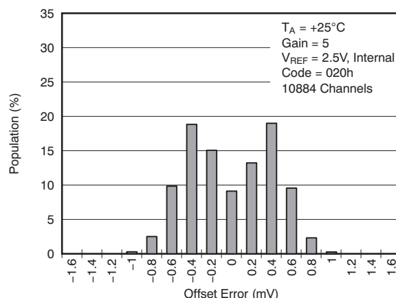
Figure 27. OFFSET VOLTAGE
