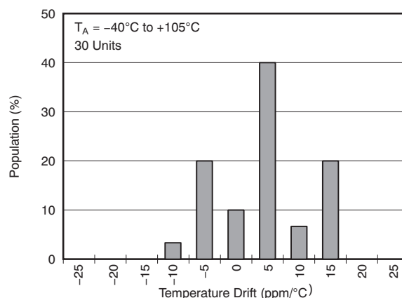
Figure 72. OUTPUT VOLTAGE DRIFT
