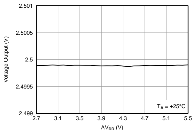
Figure 70. OUTPUT VOLTAGE vs SUPPLY
