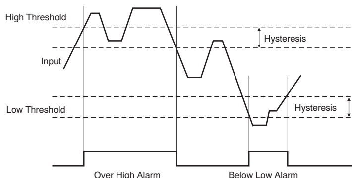
Figure 98. Hysteresis
