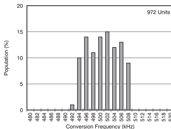
Figure 62. CONVERSION FREQUENCY
