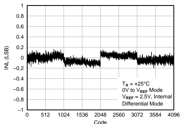
Figure 48. LINEARITY ERROR vs CODE
