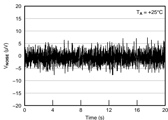
Figure 74. INTERNAL REFERENCE NOISE (0.1 Hz to 10 Hz)
