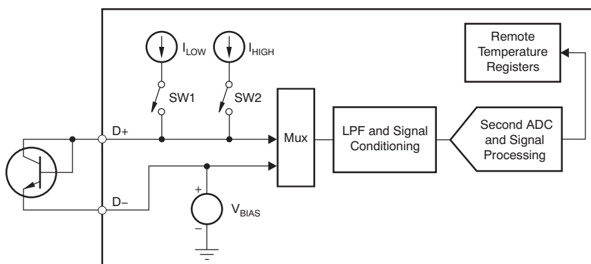
Figure 87. Remote Temperature Sensor
