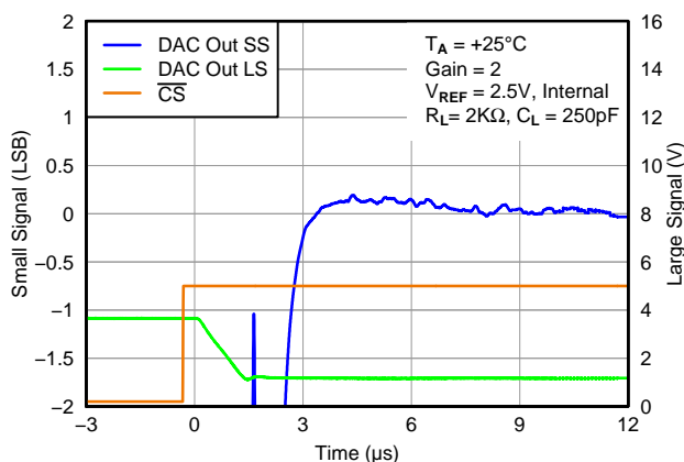
Figure 42. SETTLING TIME FALLING EDGE
