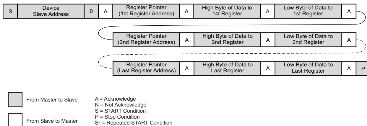
Figure 101. Write to Multiple 16-Bit Registers
