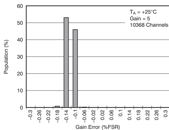
Figure 21. GAIN ERROR
