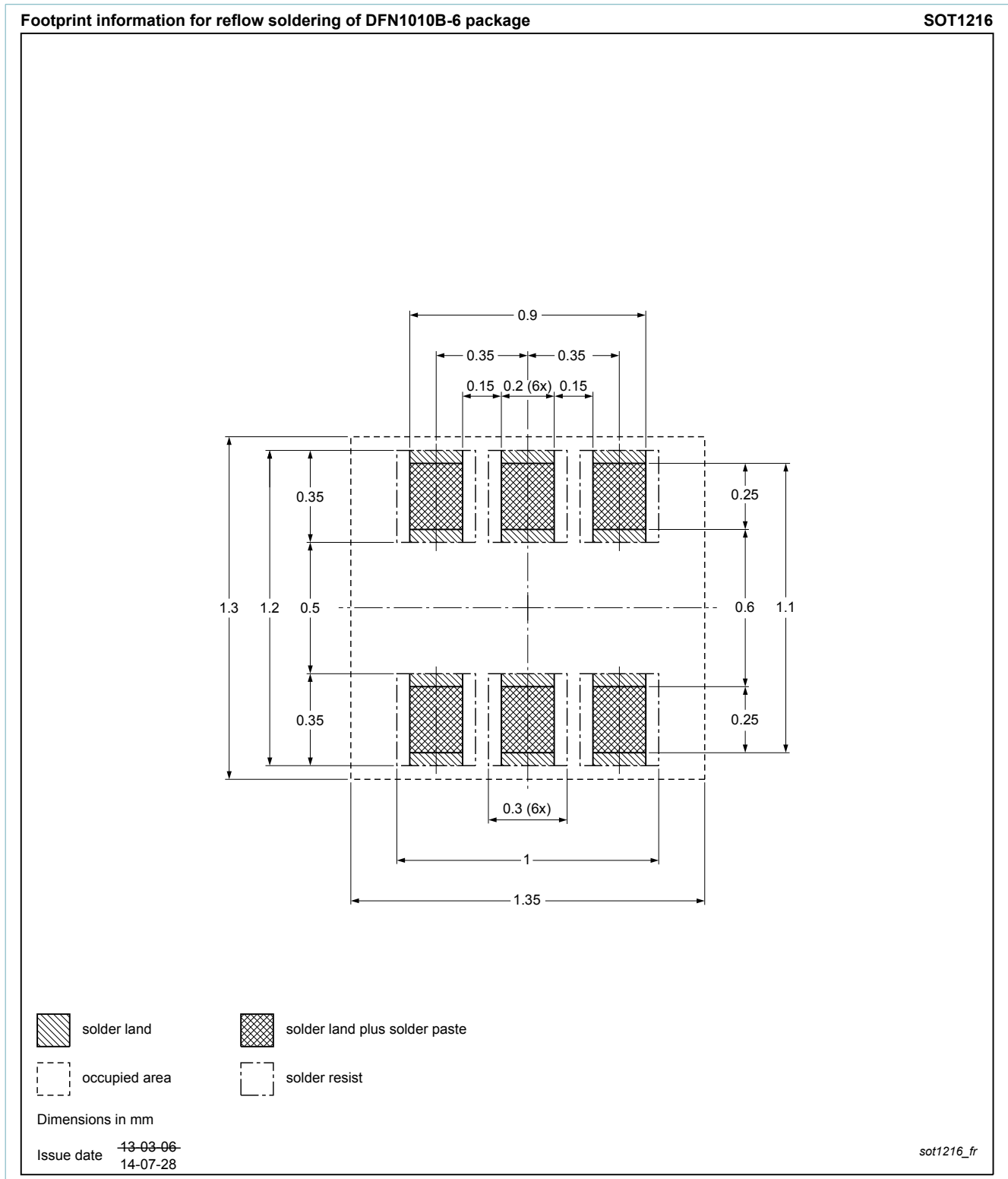
Fig. 17. Reflow soldering footprint for DFN1010B-6 (SOT1216)
