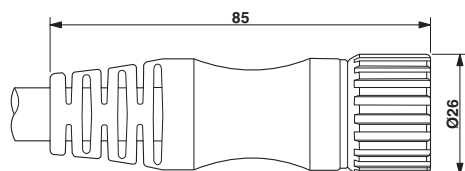
Dimensioned drawing
