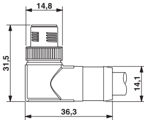
Dimensioned drawing
