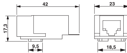
RJ45 socket insert
