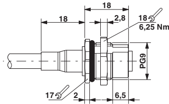
Dimensioned drawing
